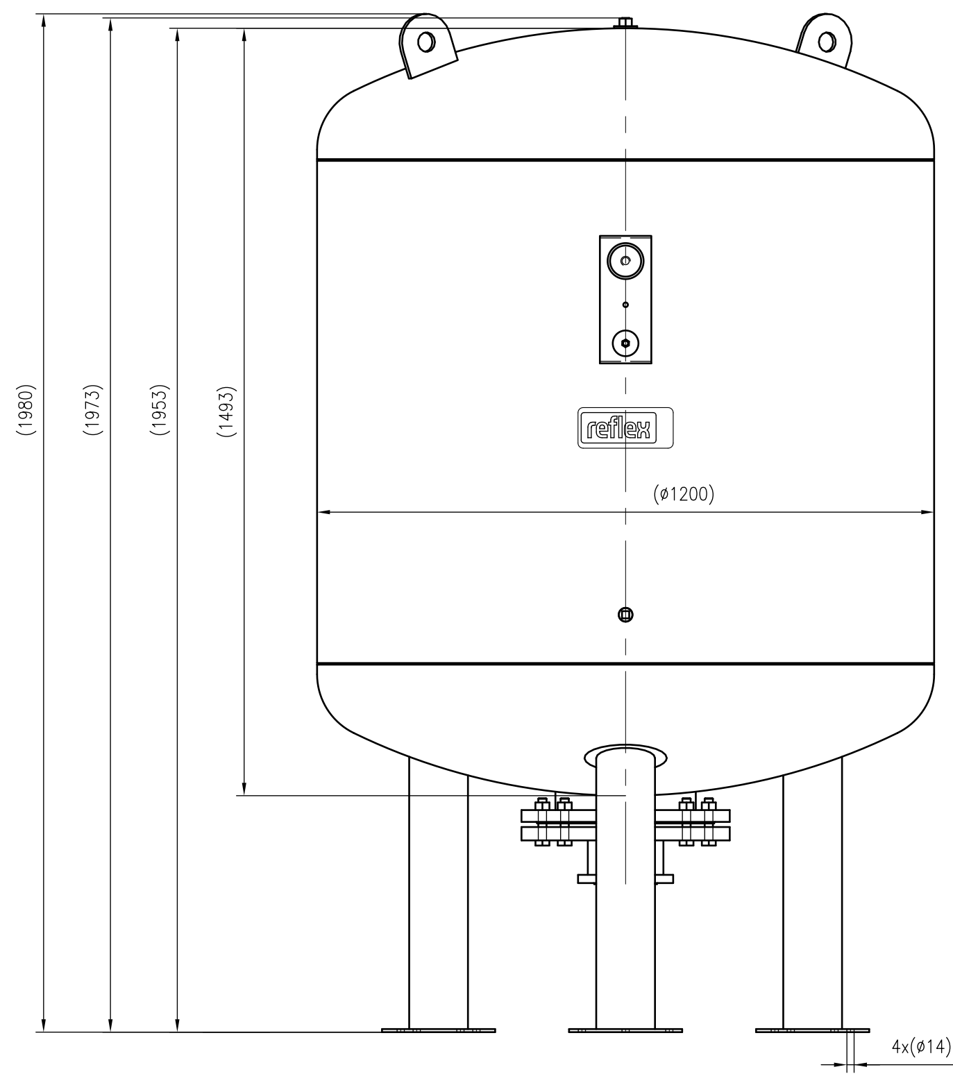
Front view
