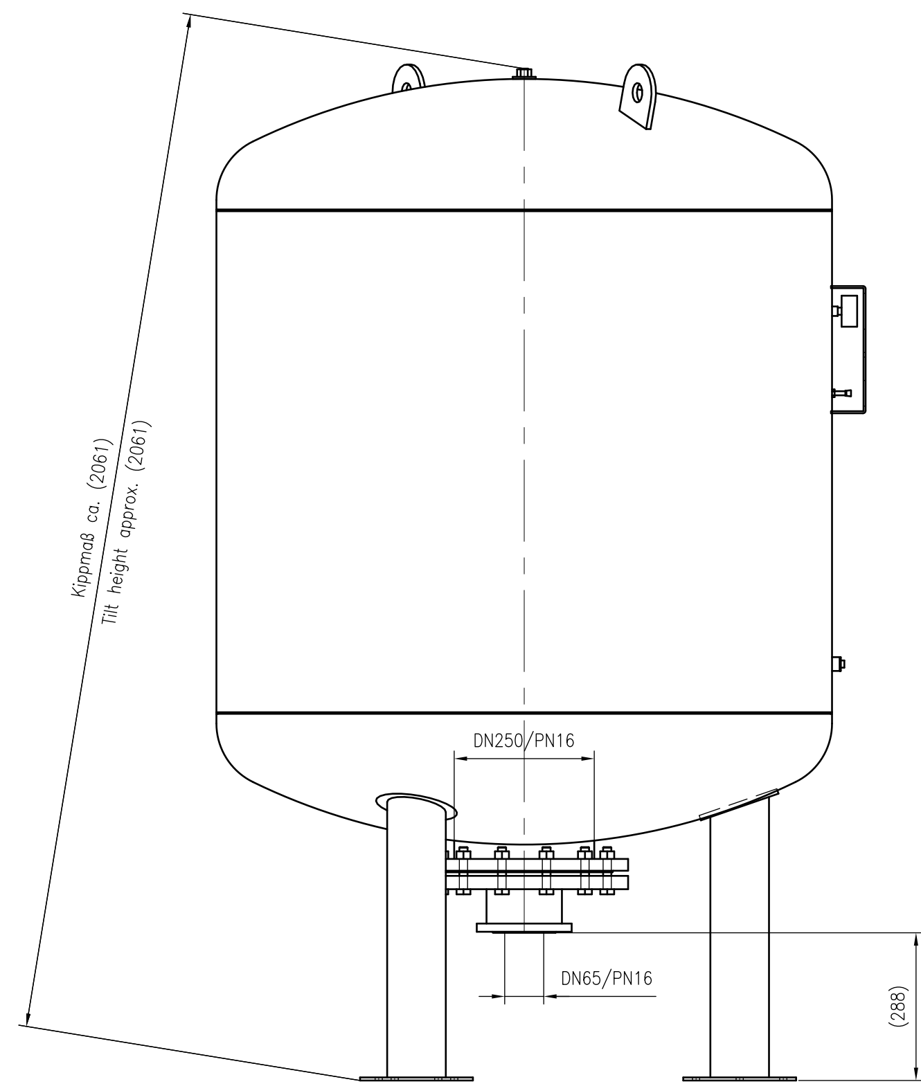
Side view
