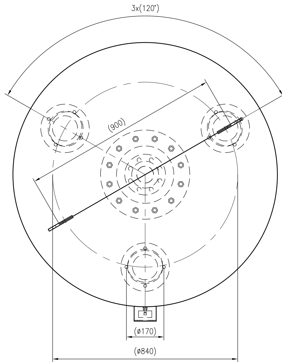
Top view
