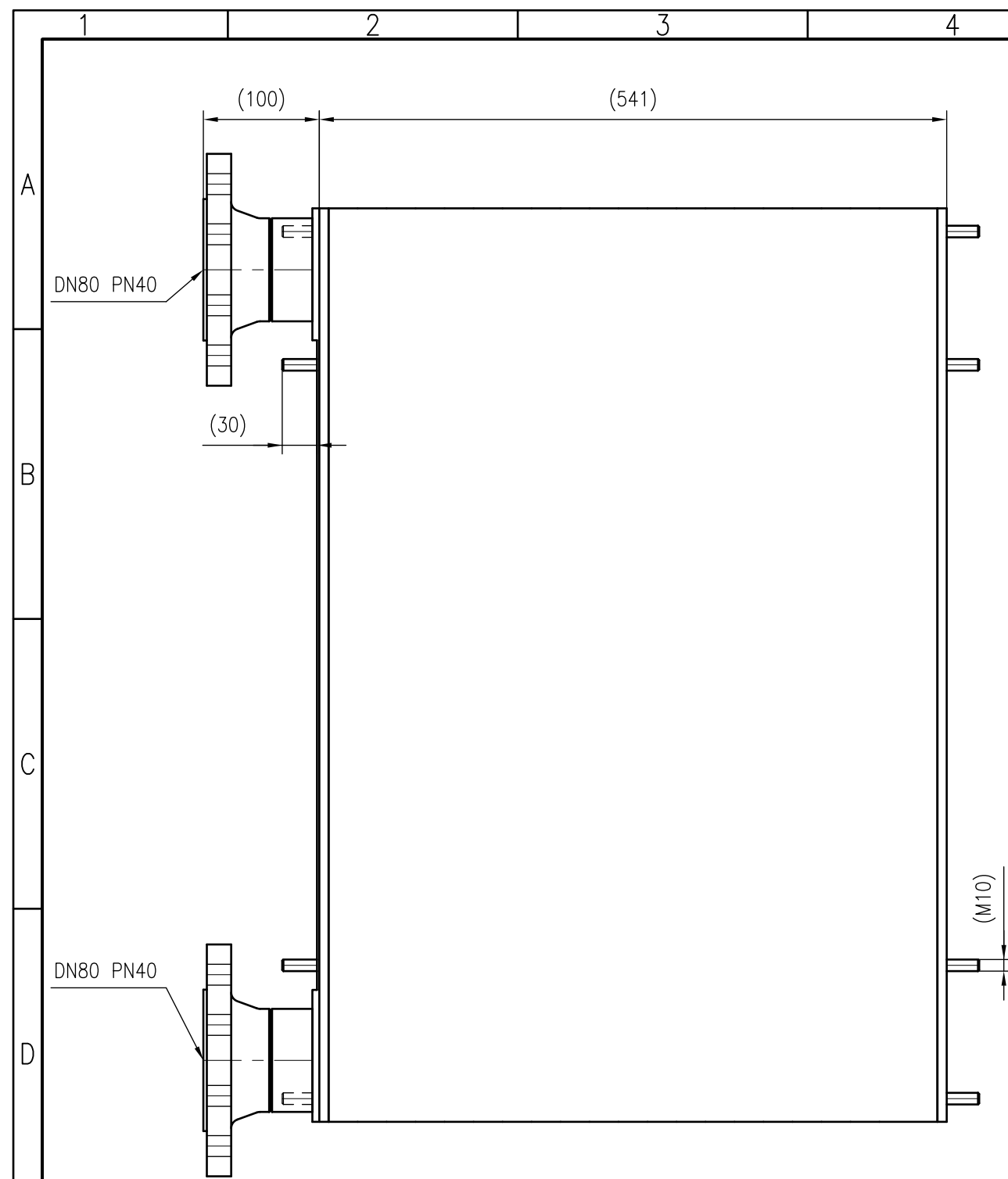
Side view
