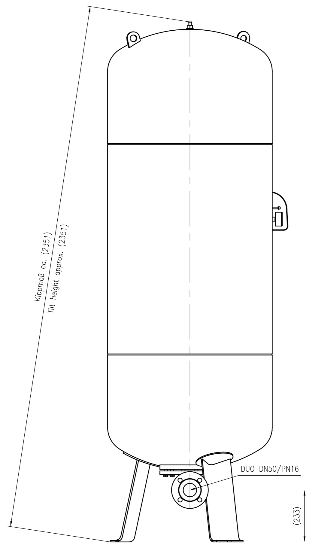
Side view
