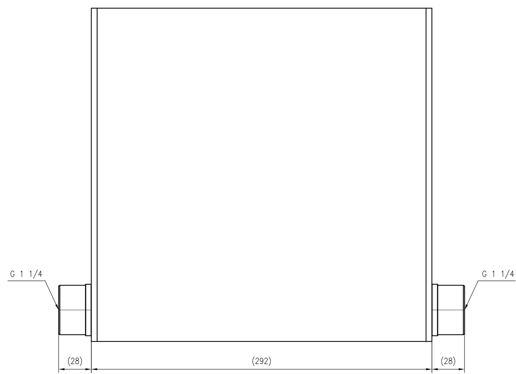
Side view
