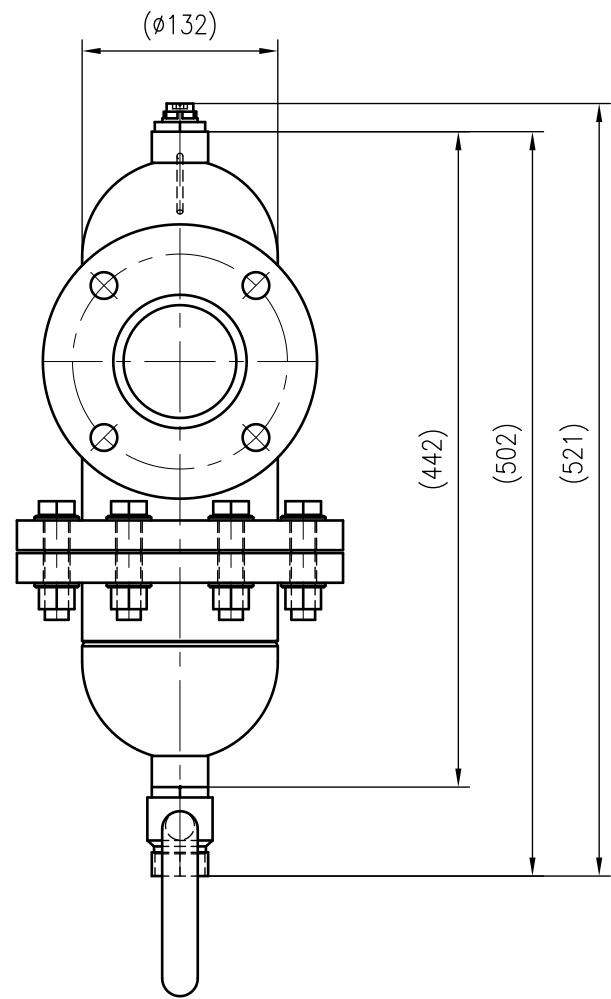
Side view
