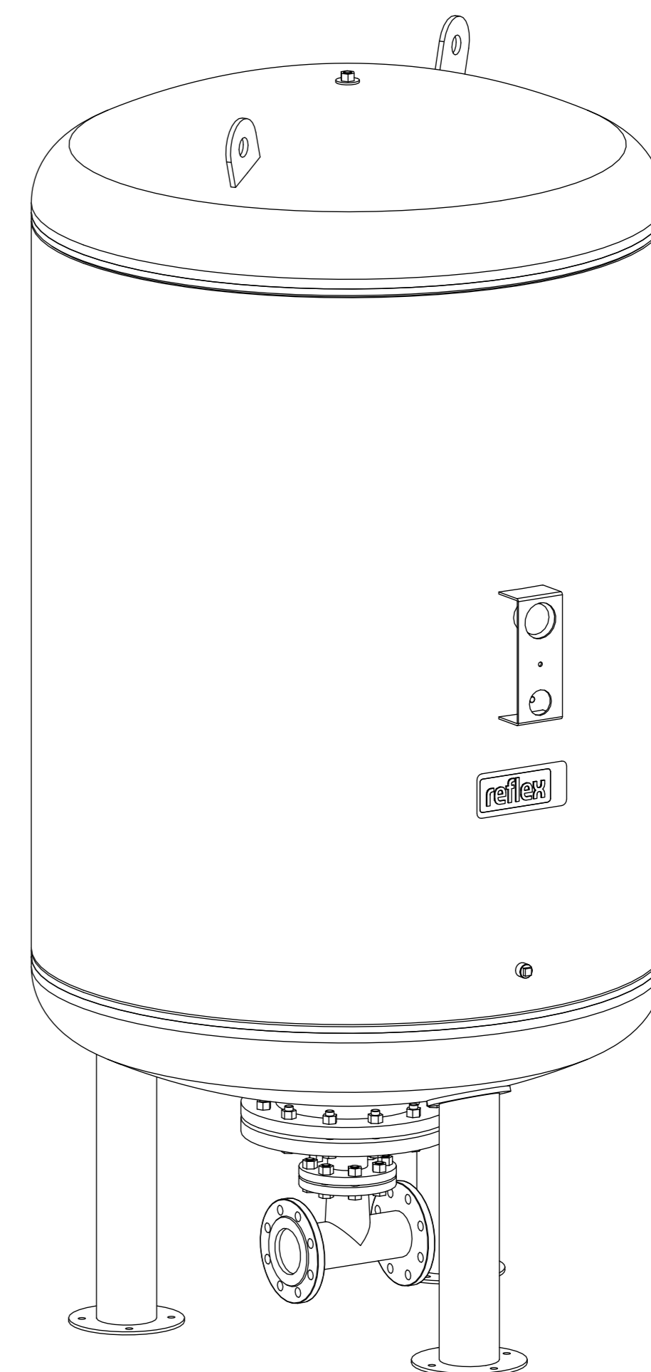
Isometric view
