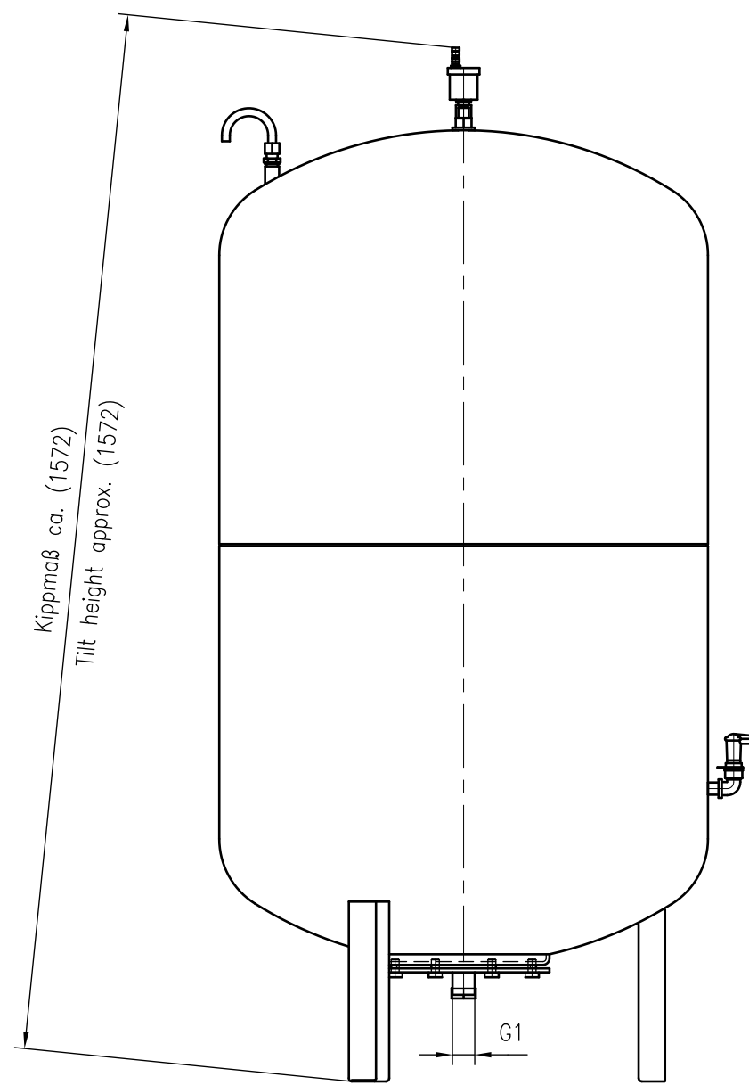
Side view
