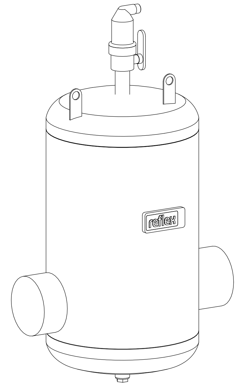
Isometric view
