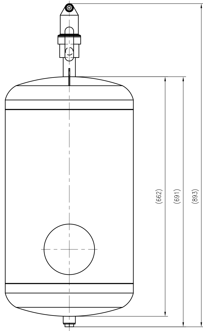
Side view
