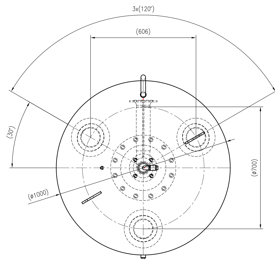
Top view
