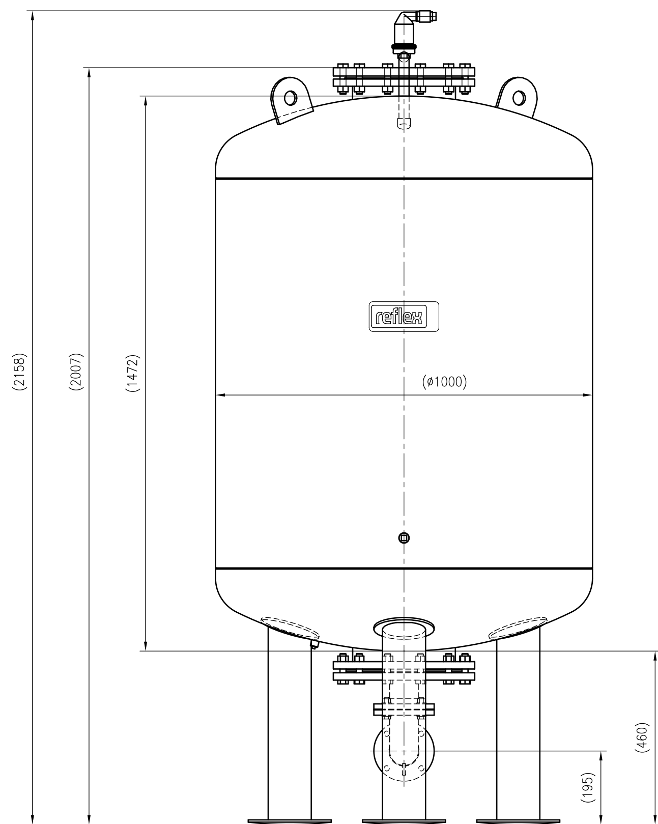
Front view
