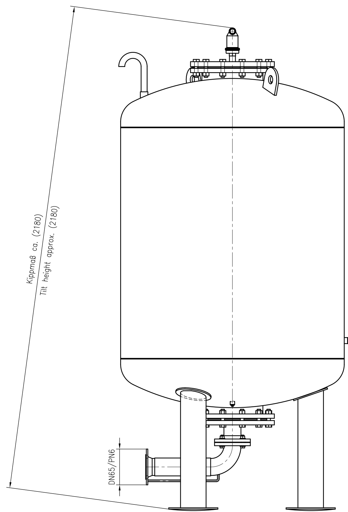
Side view
