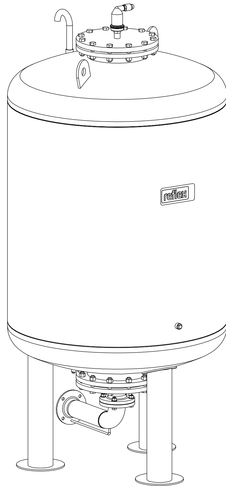
Isometric view
