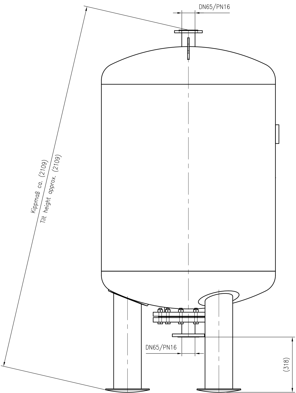
Side view
