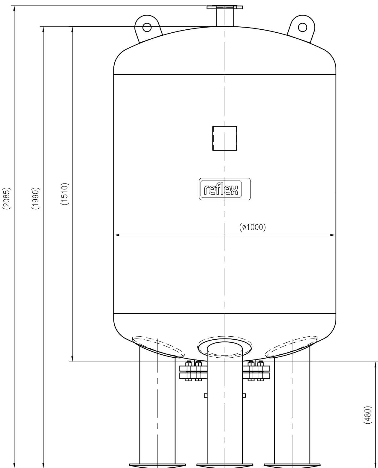
Front view
