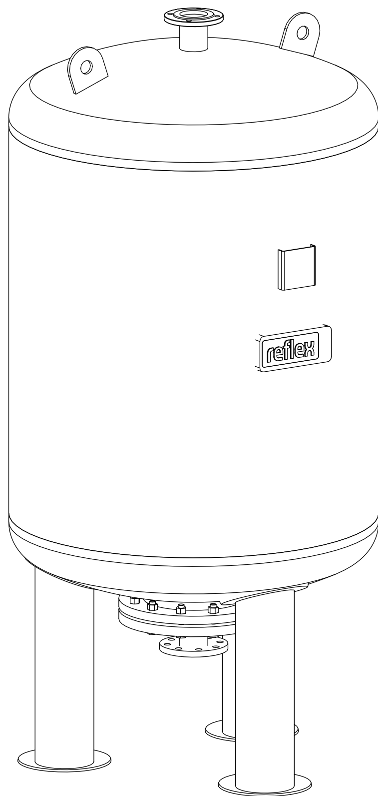
Isometric view
