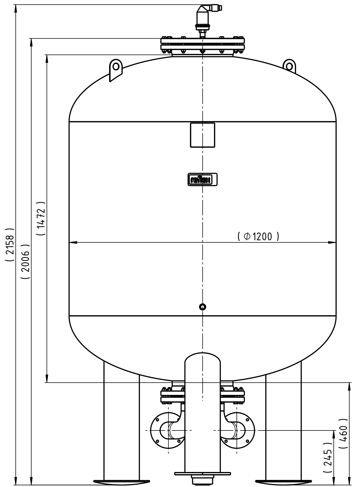
Front view
