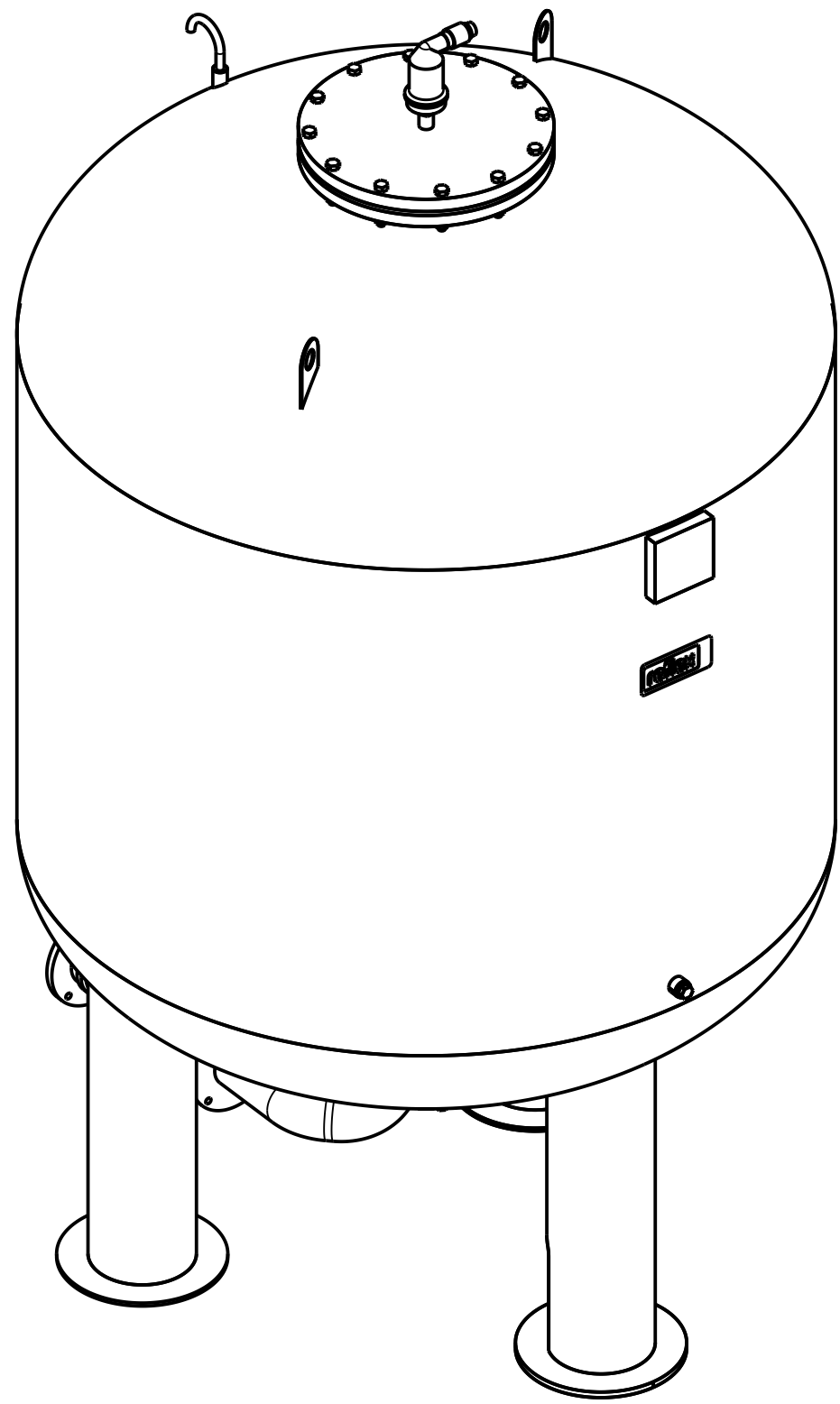
Isometric view
