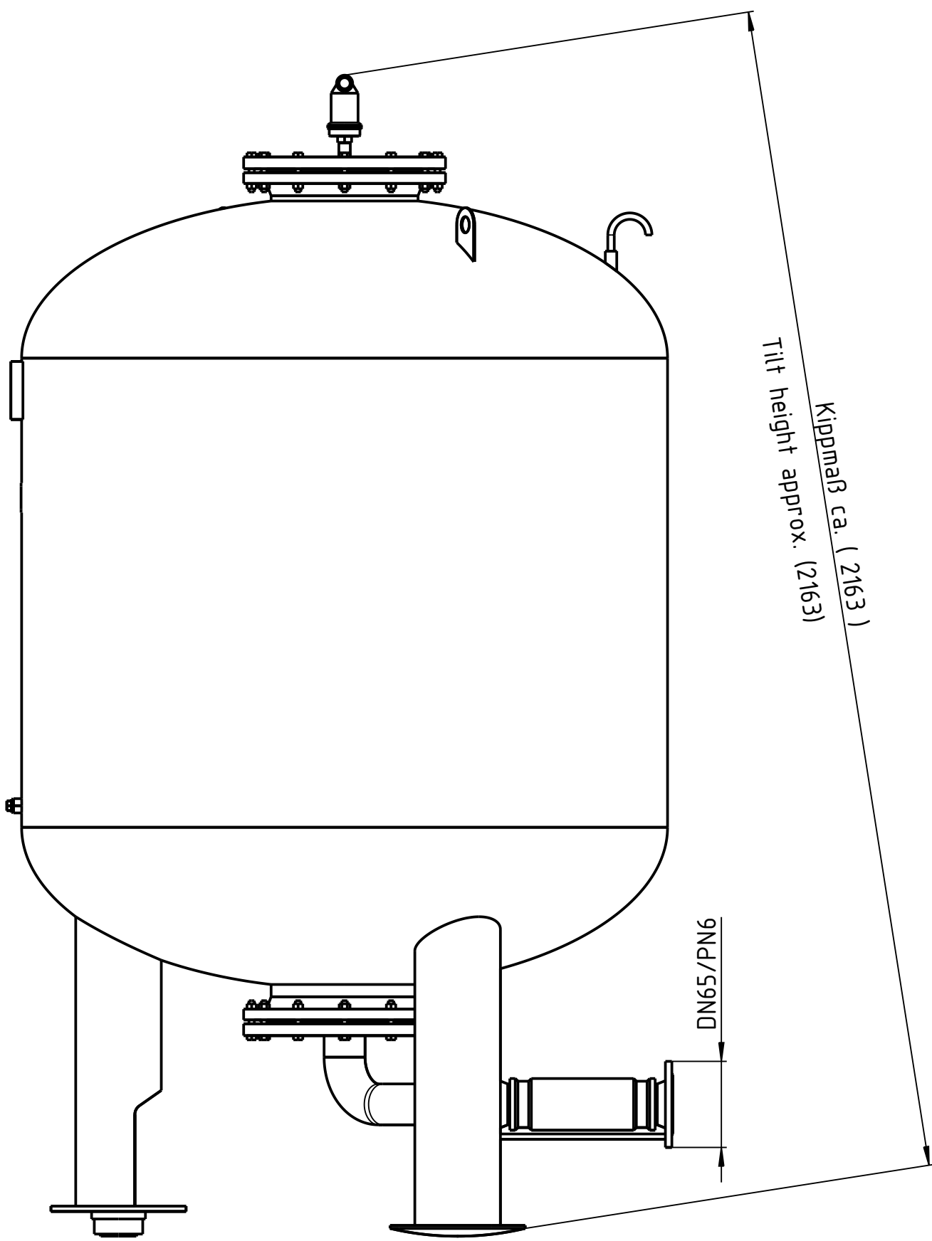
Right view
