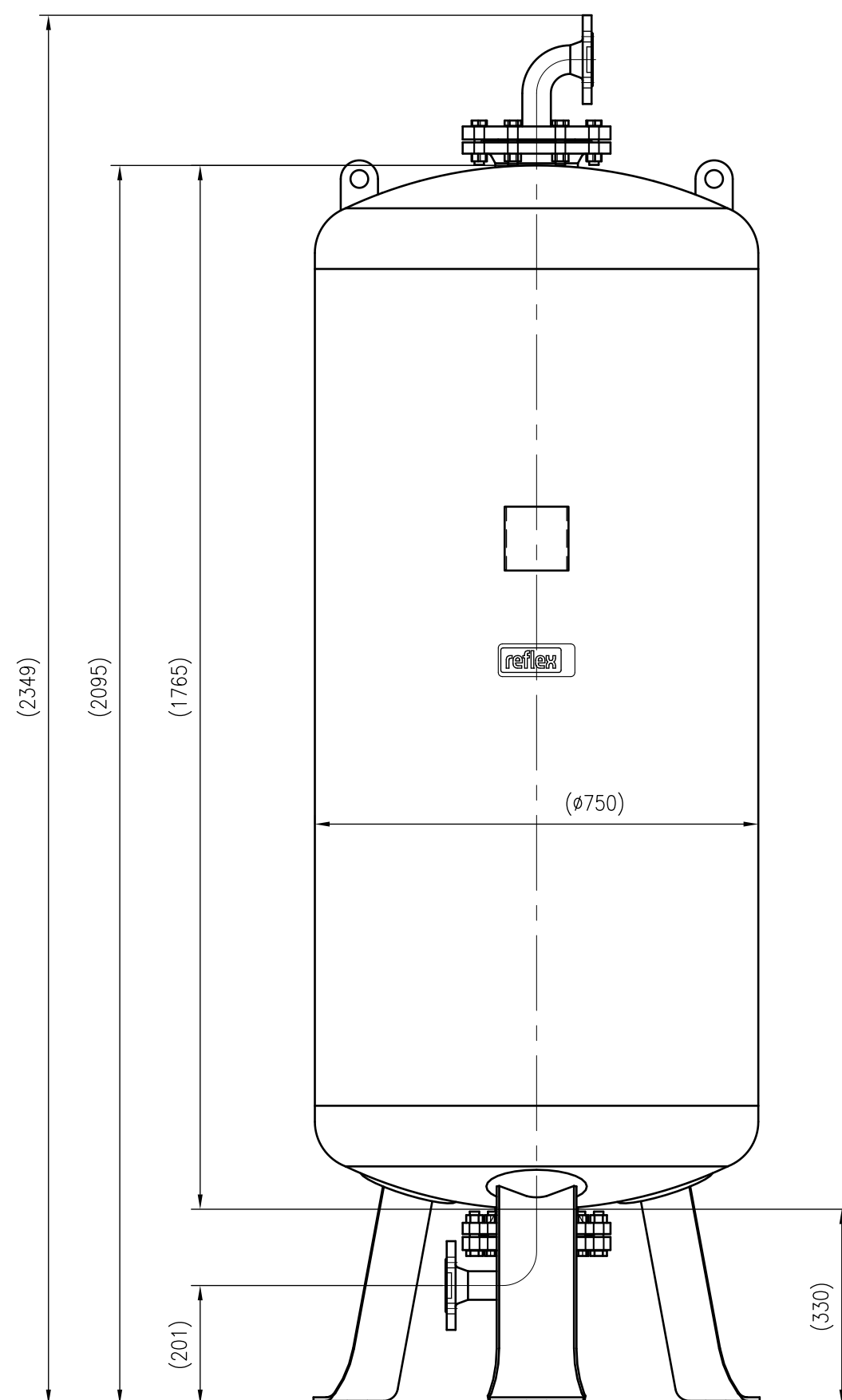
Front view
