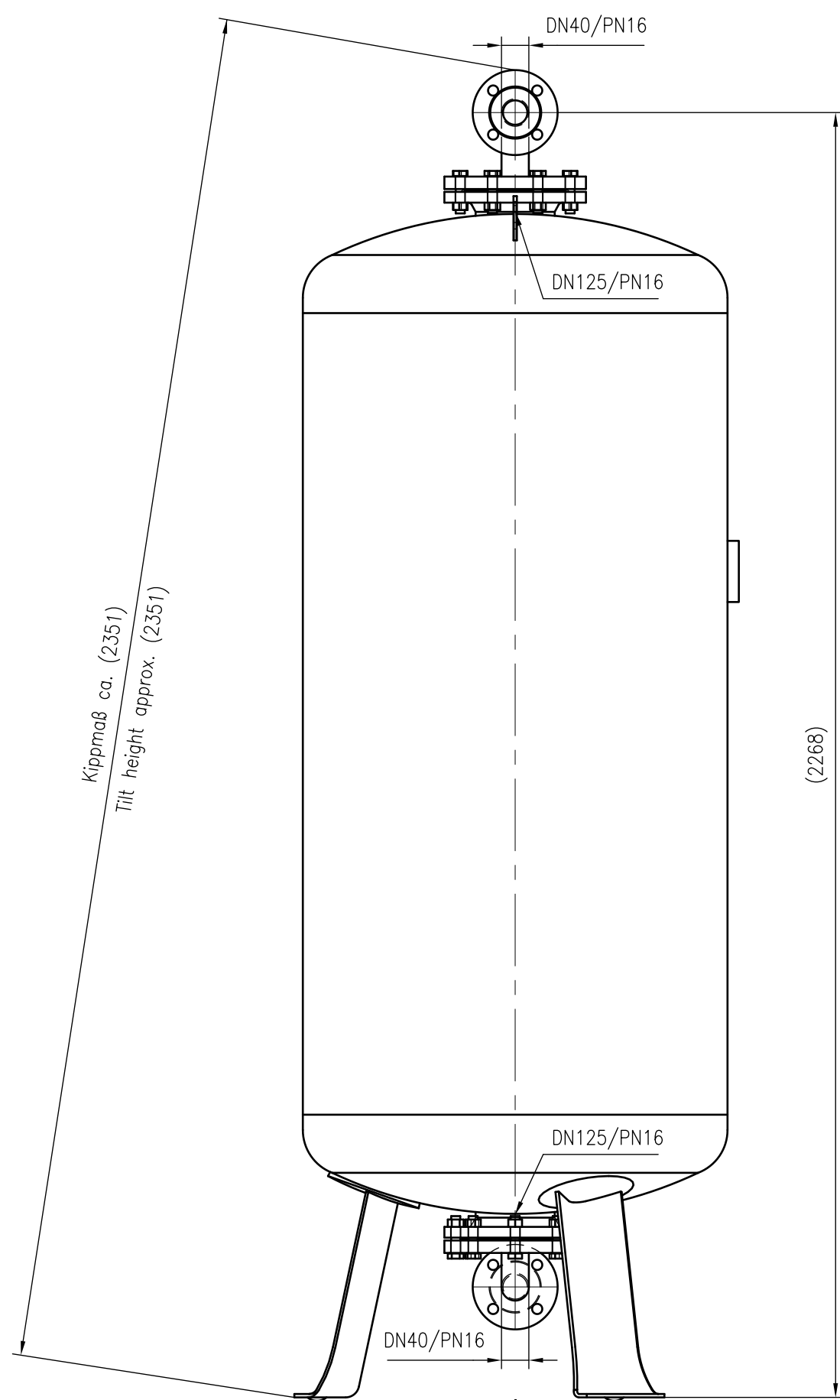
Side view
