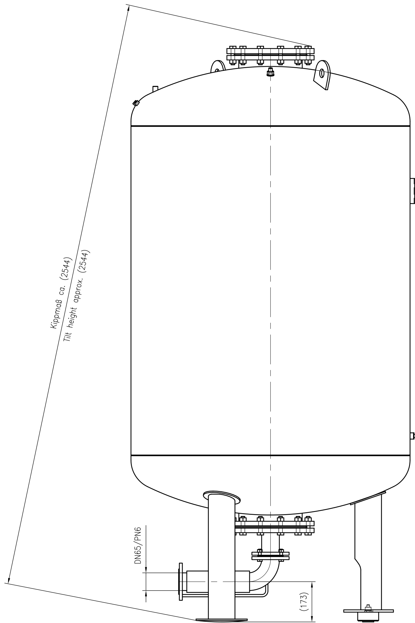
Side view
