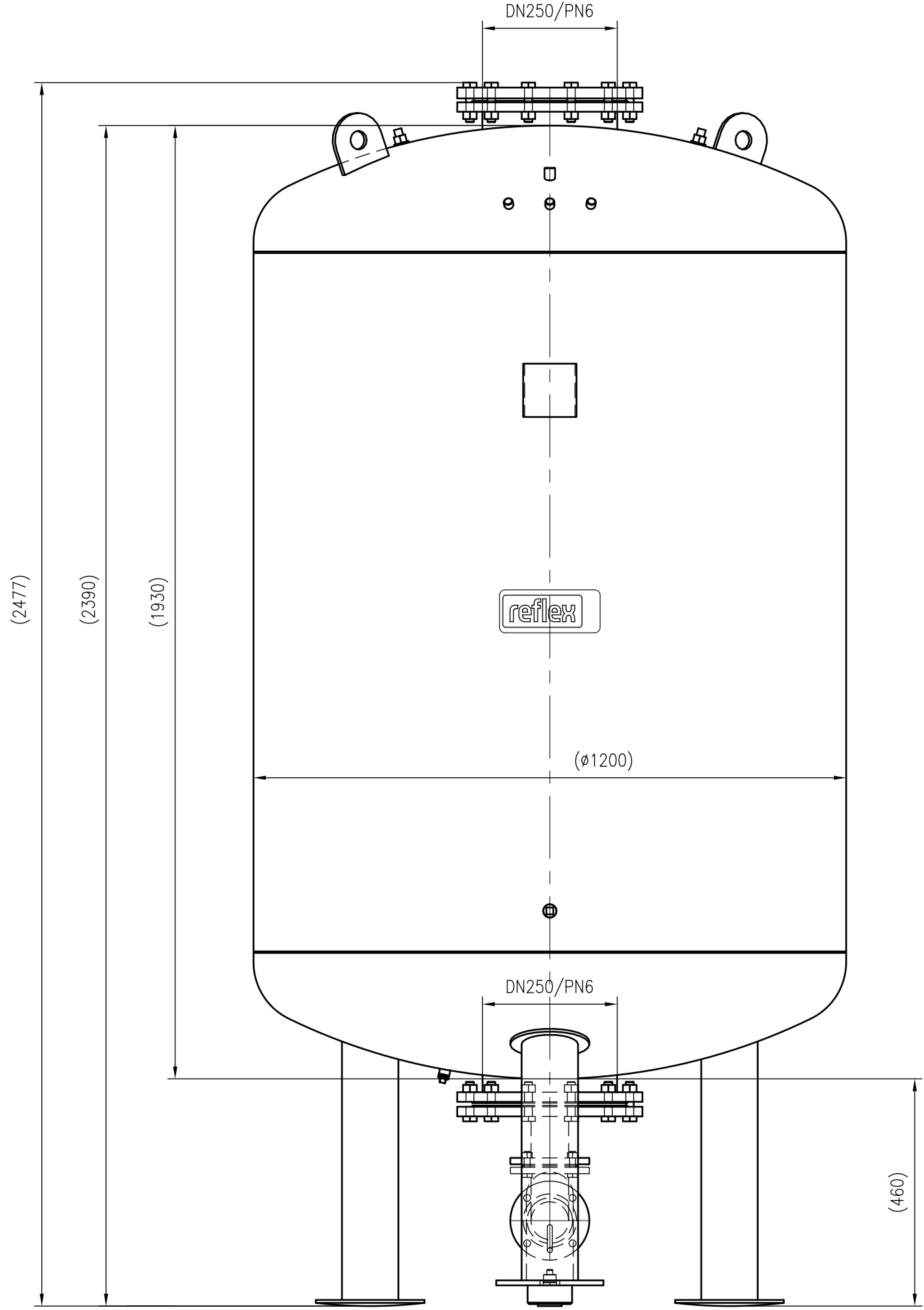
Front view
