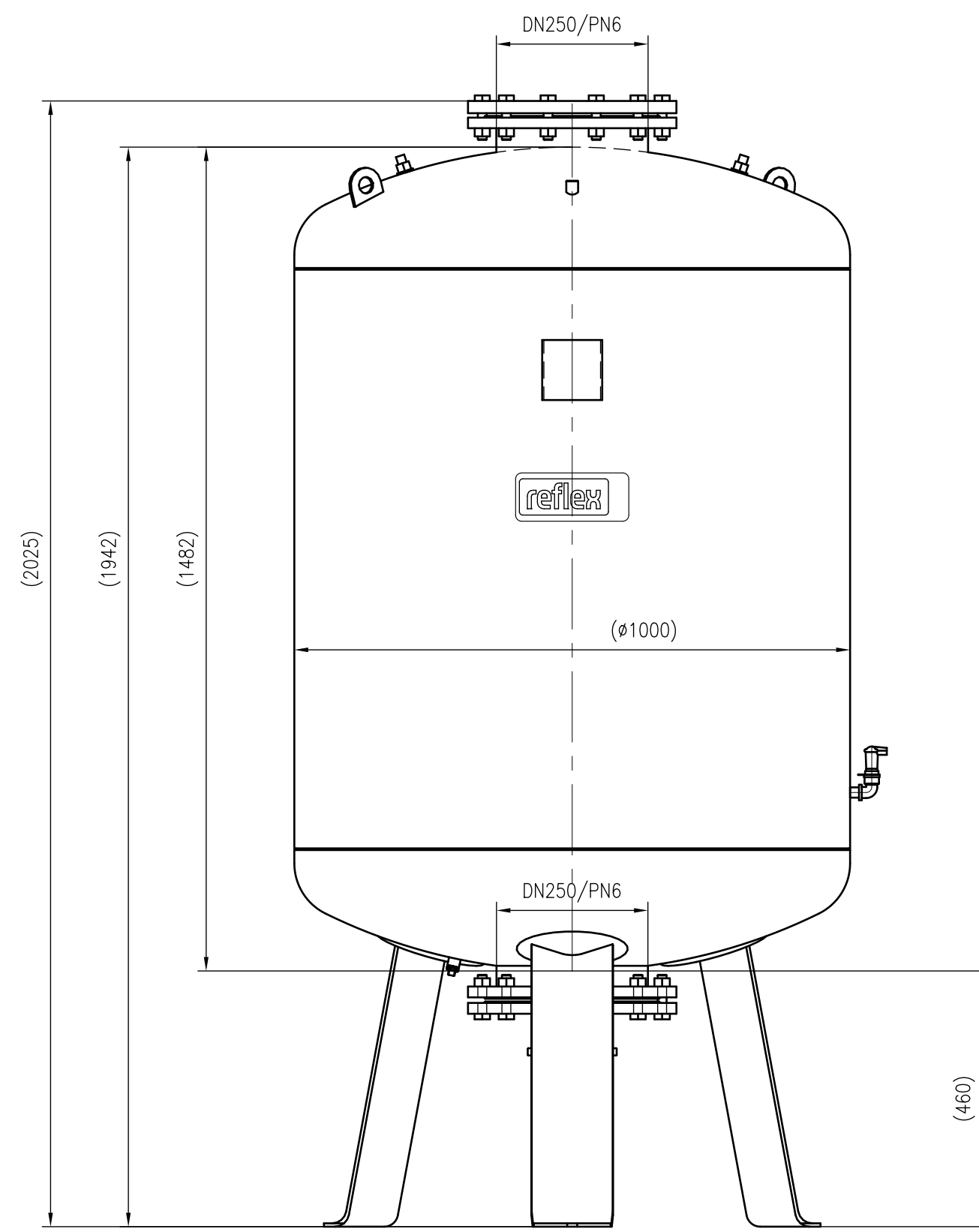
Front view
