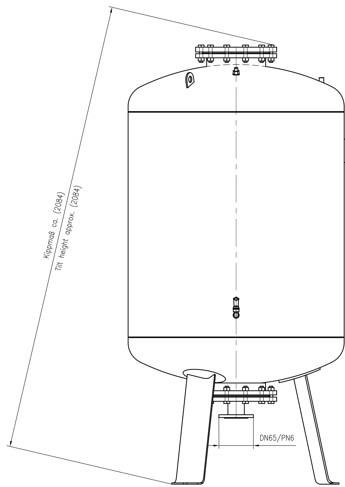
Side view
