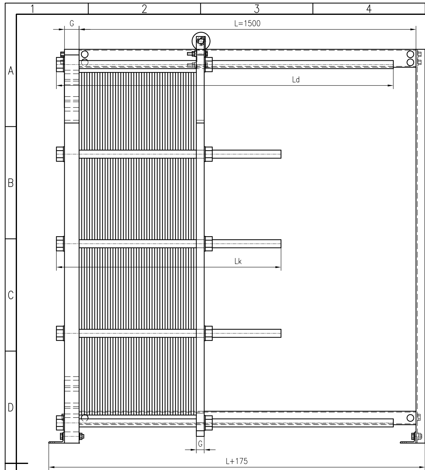
Side view
