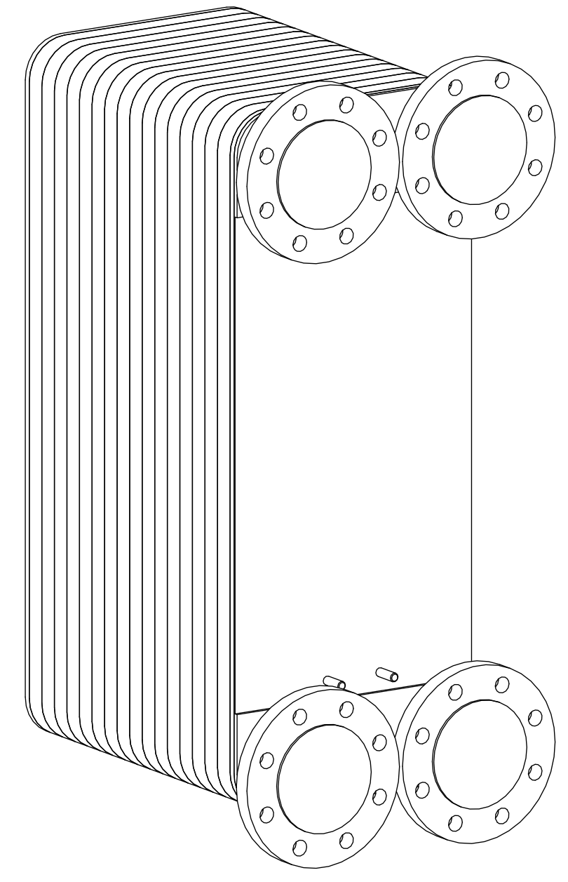
Isometric view
