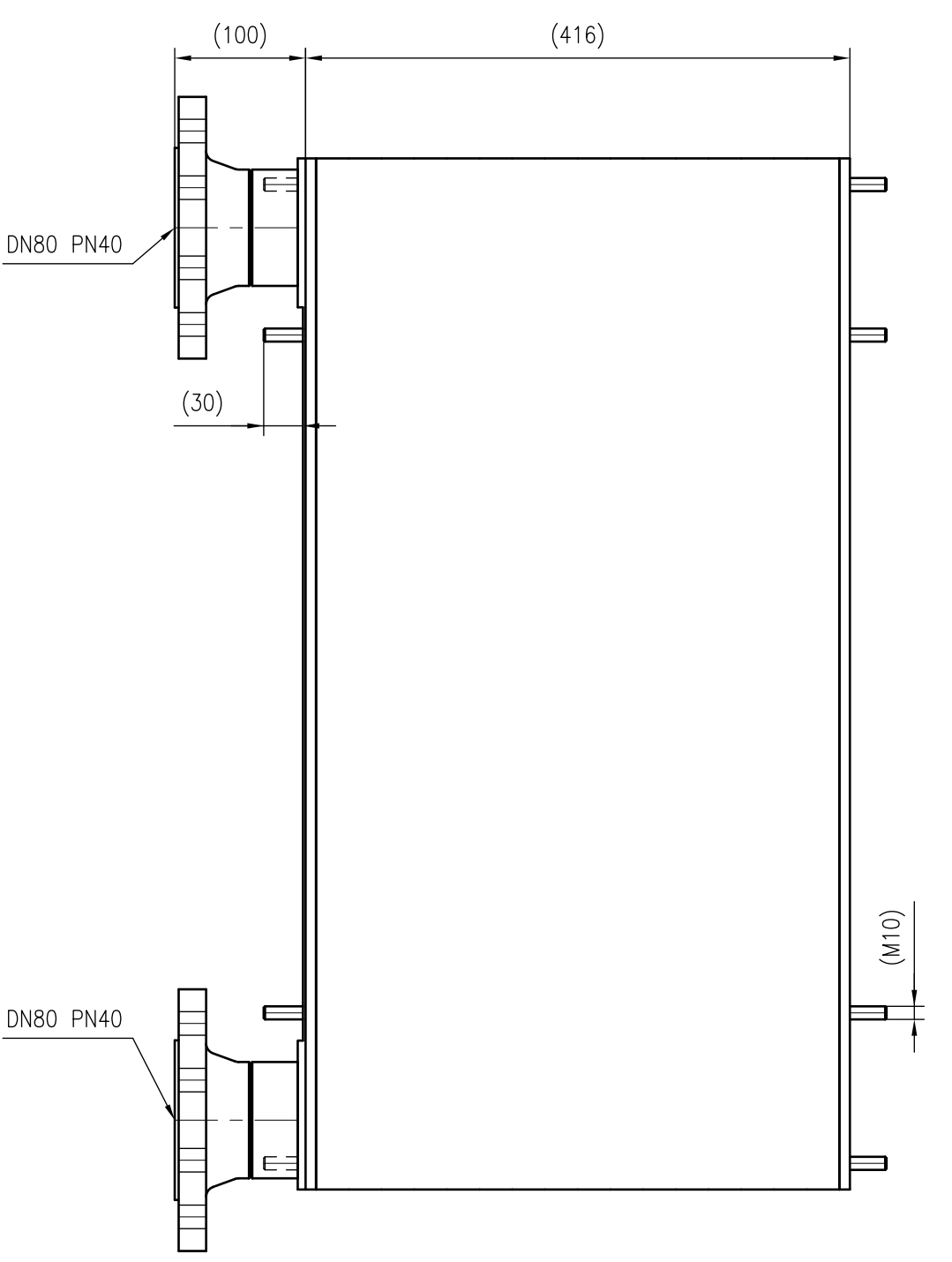
Side view
