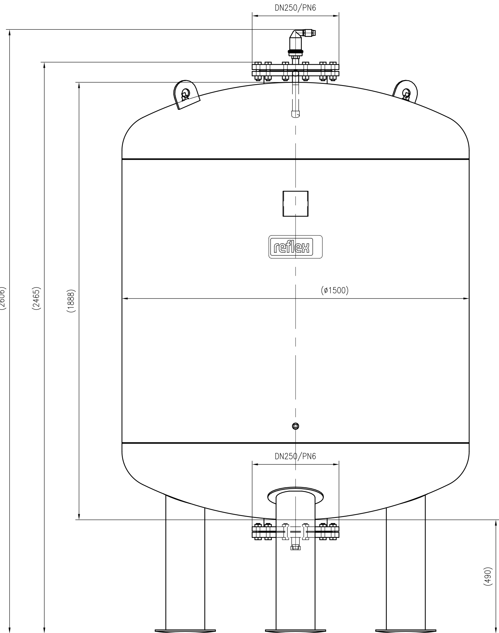
Front view
