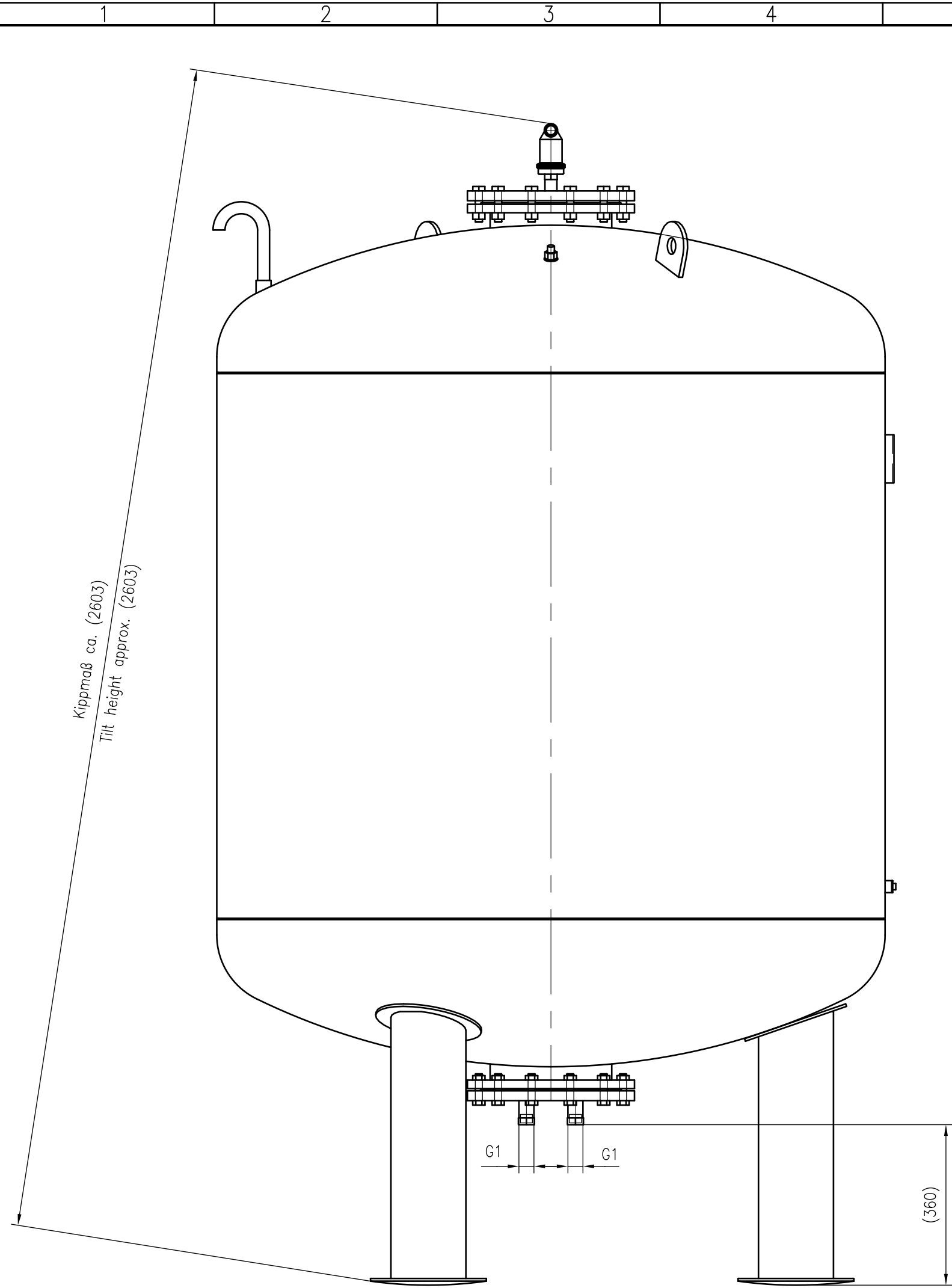
Side view
