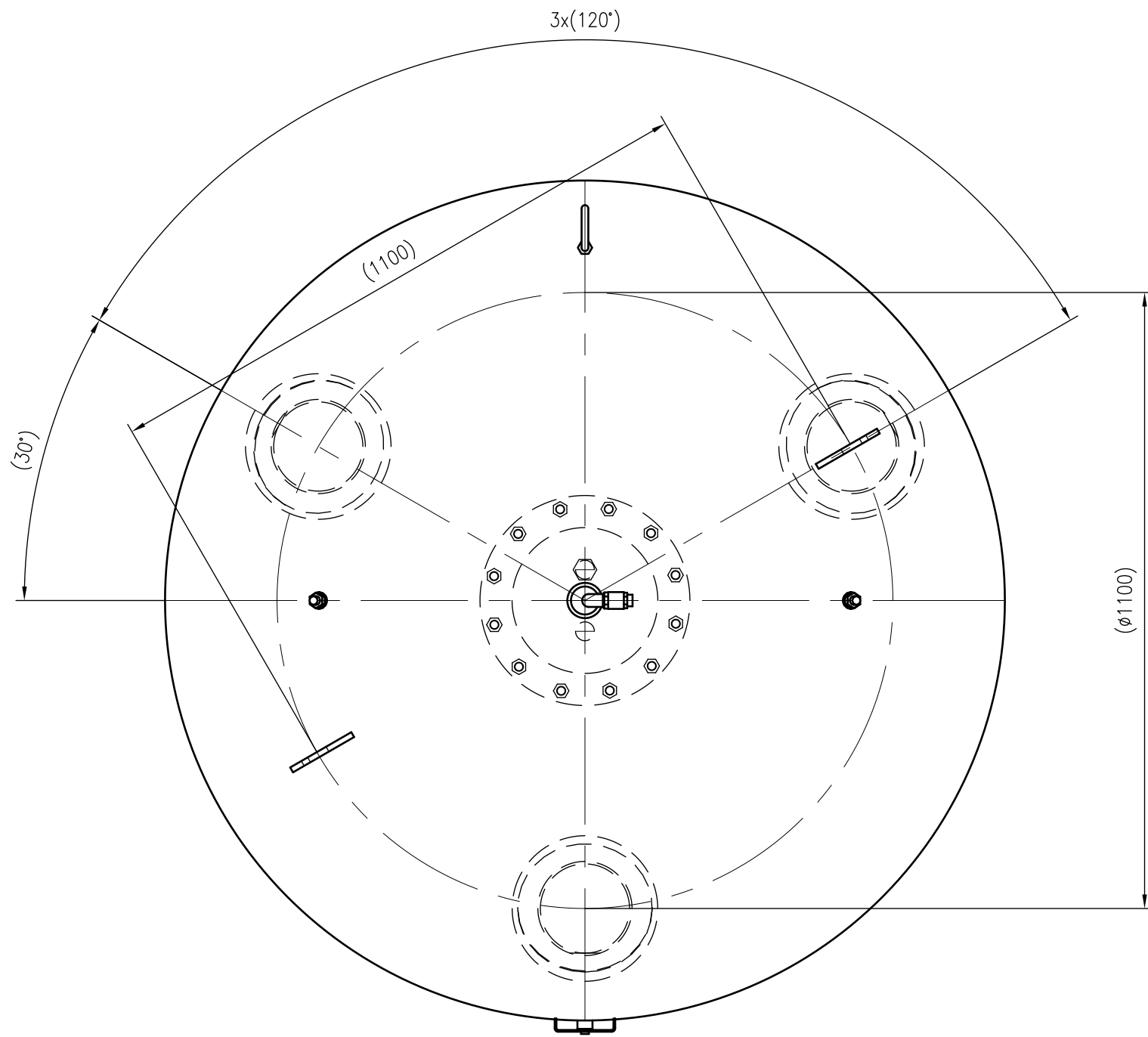
Top view
