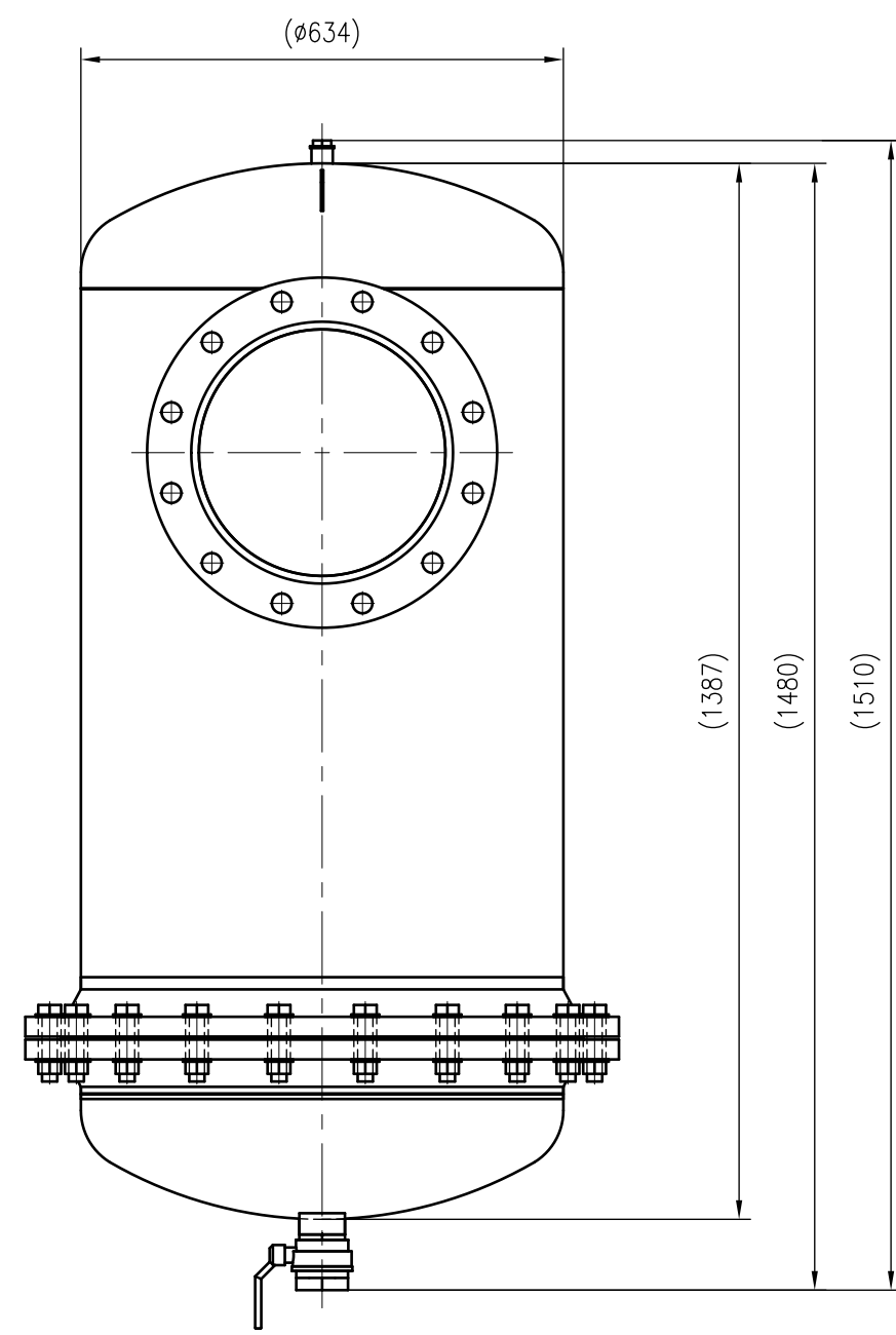
Side view
