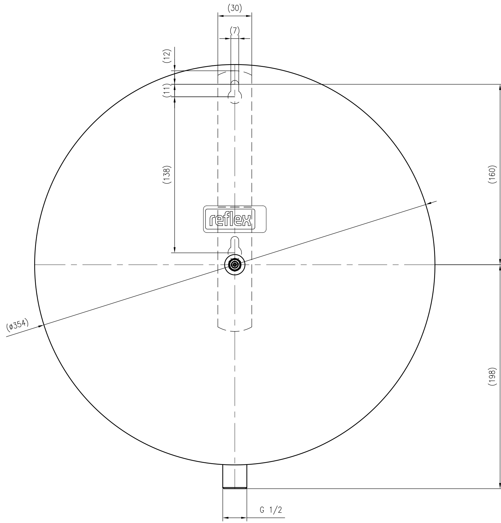
Front view
