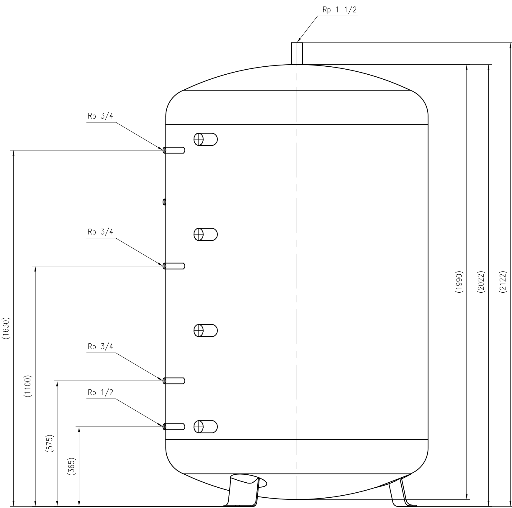
Side view
