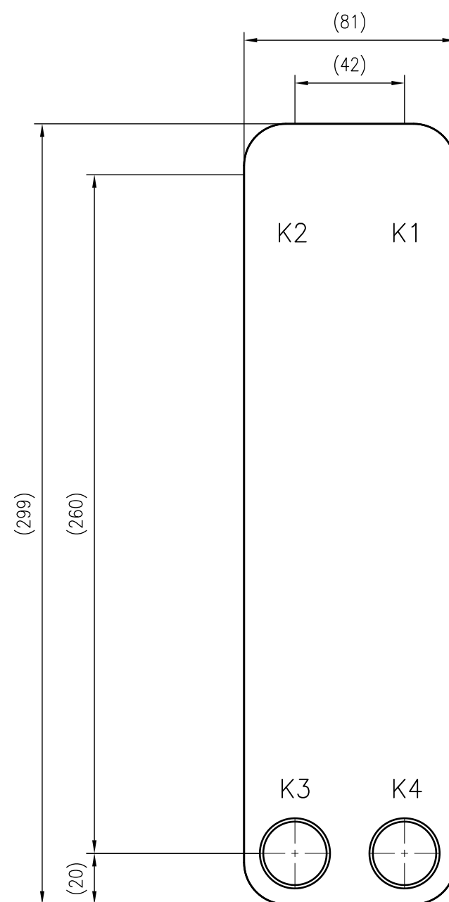
Front view
