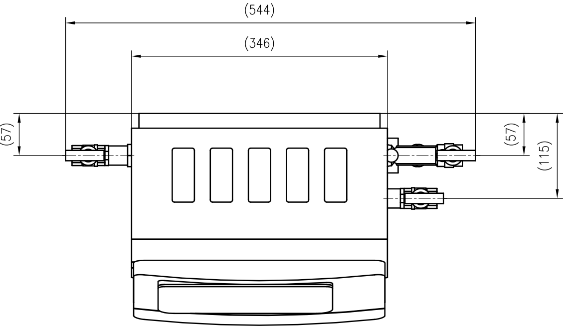
Top view
