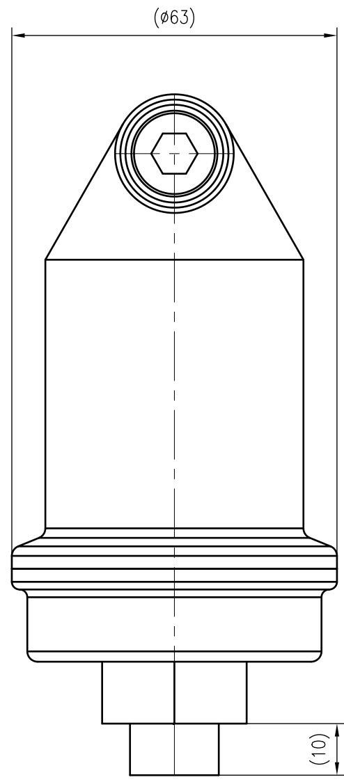
Side view
