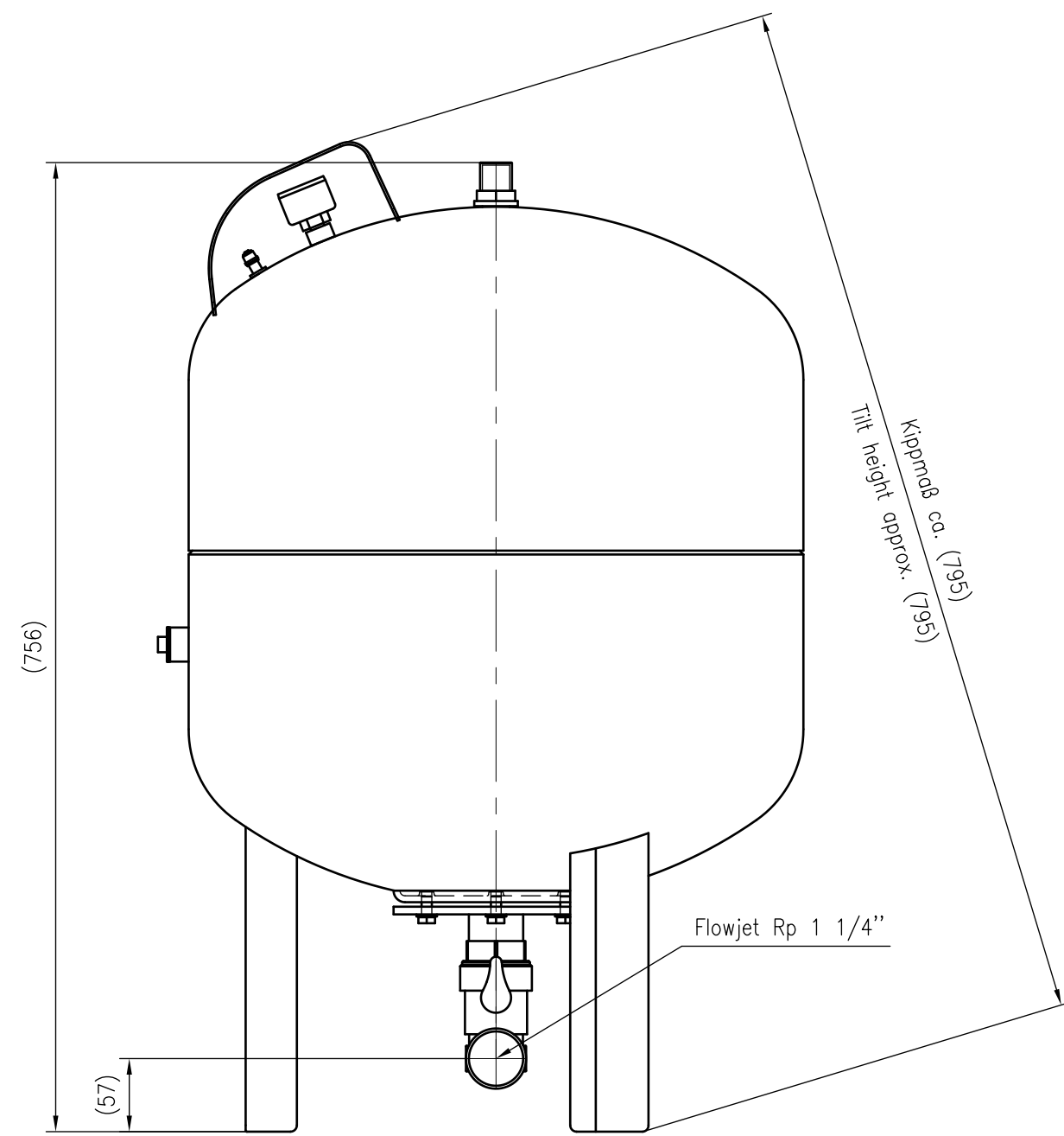
Side view
