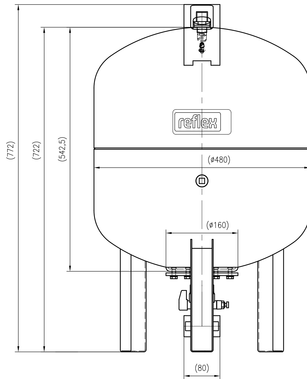
Front view
