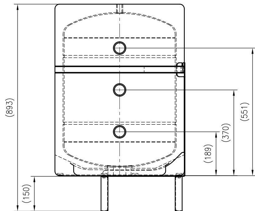
Side view
