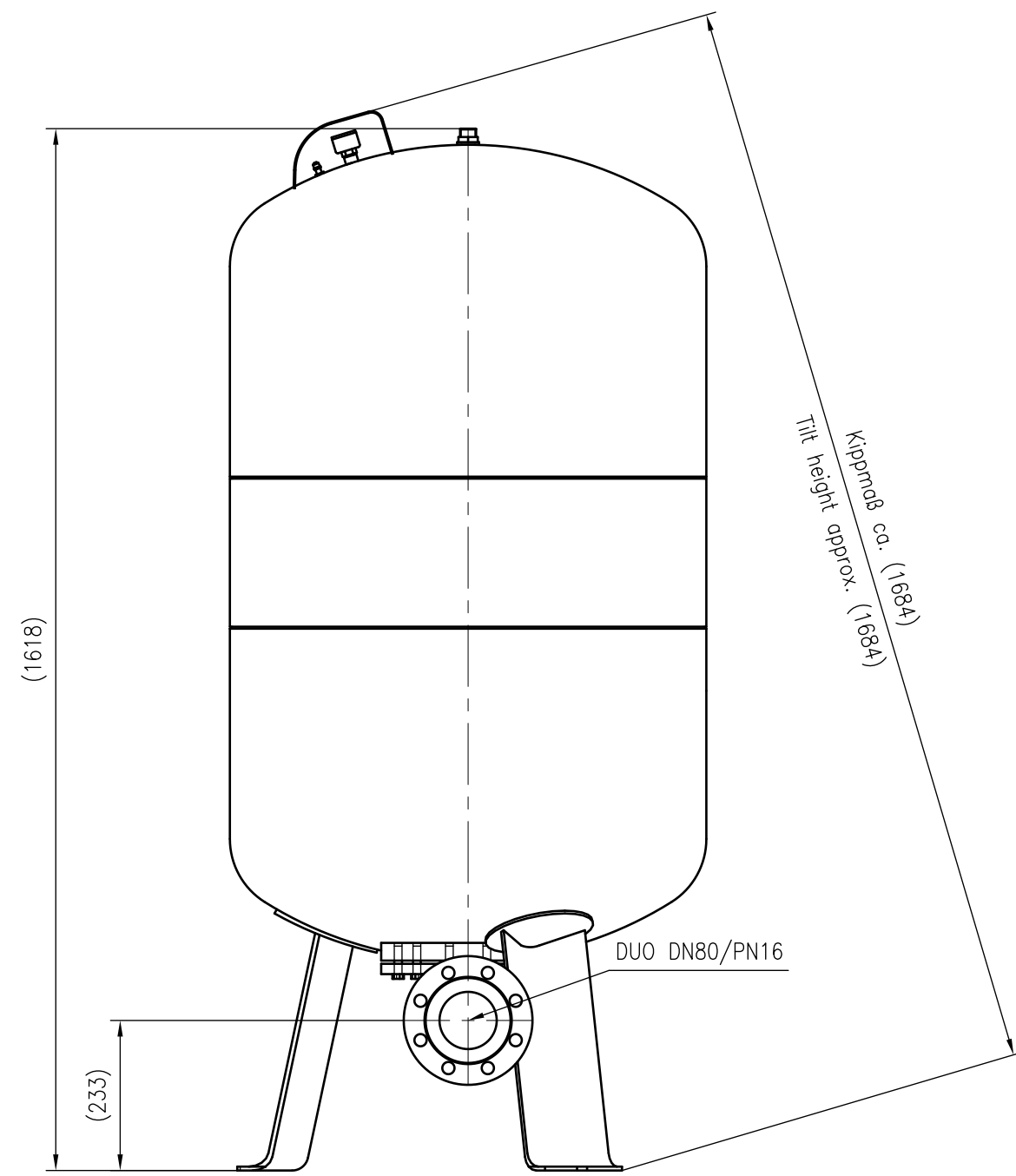
Side view
