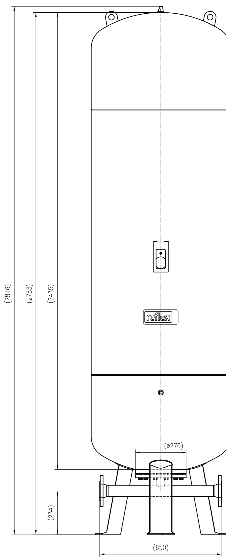
Front view
