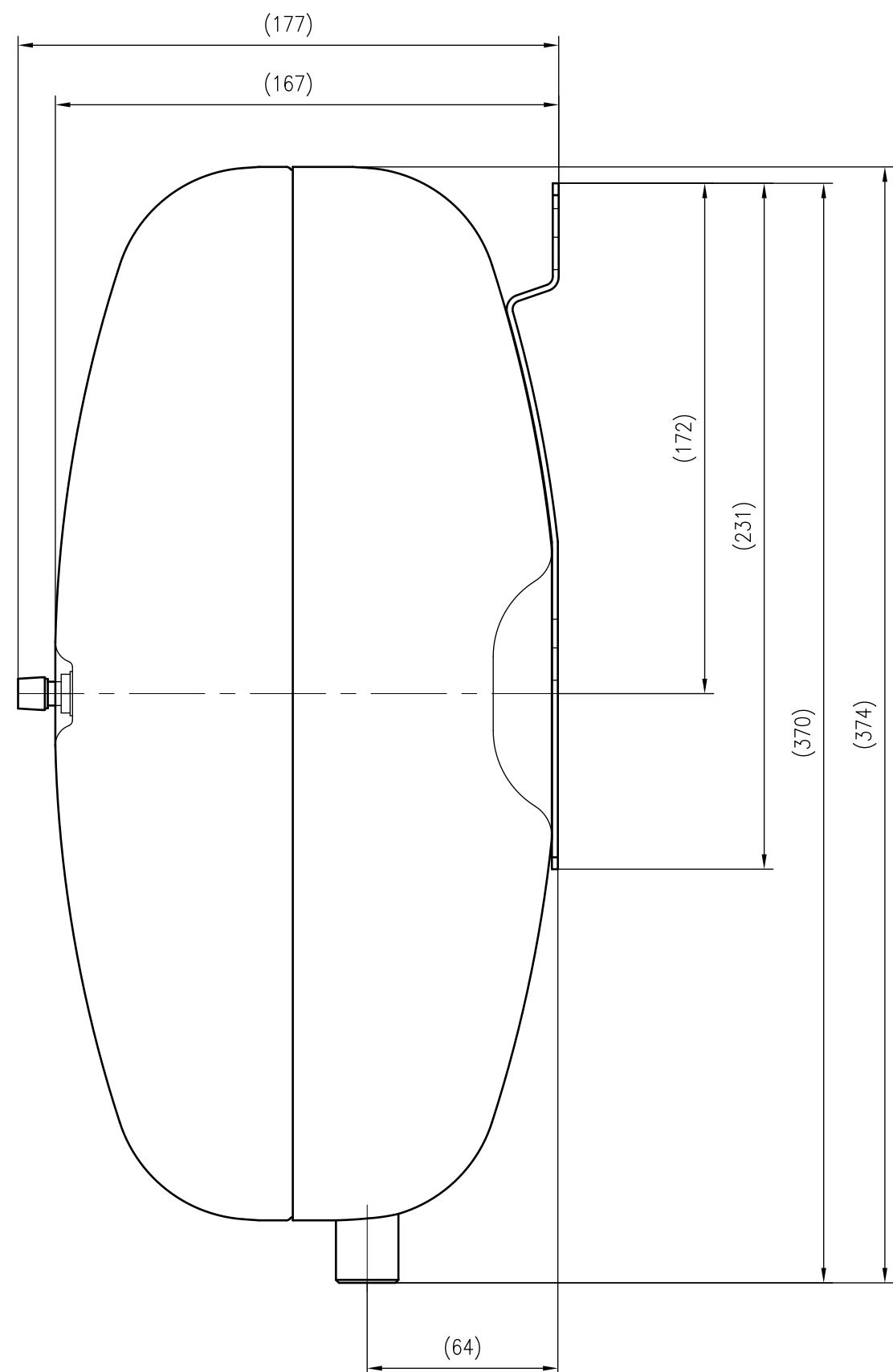
Side view
