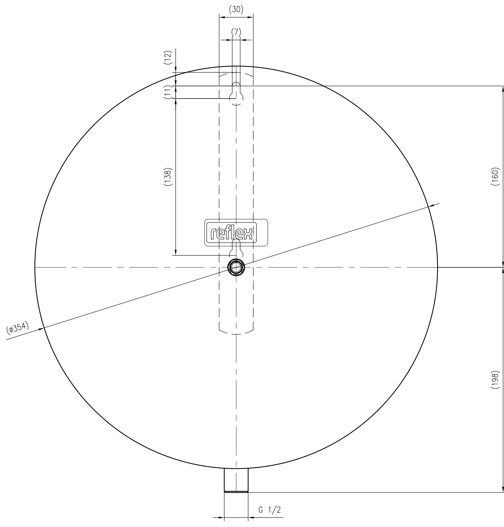
Front view
