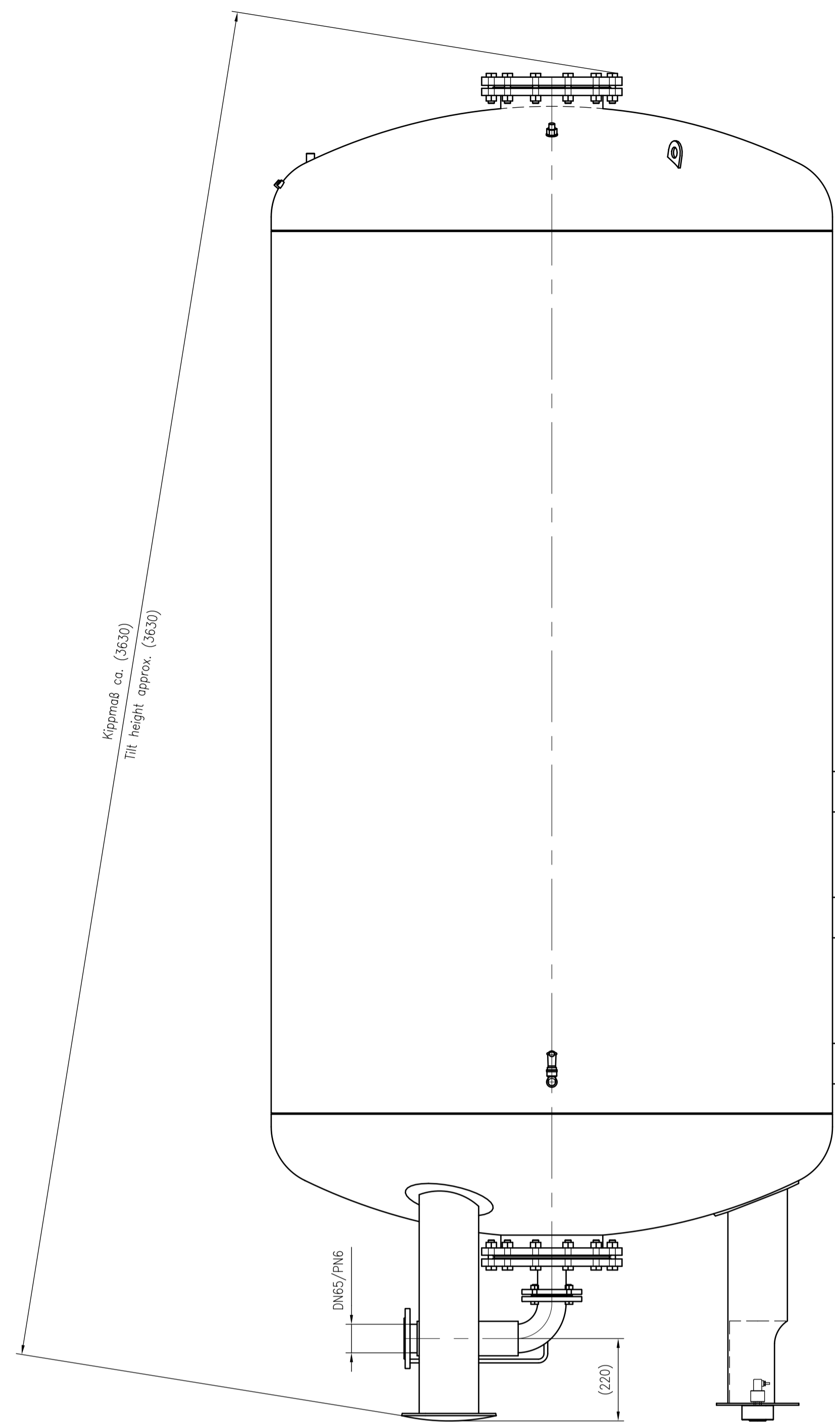
Side view
