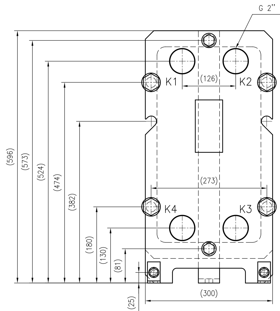
Front view
