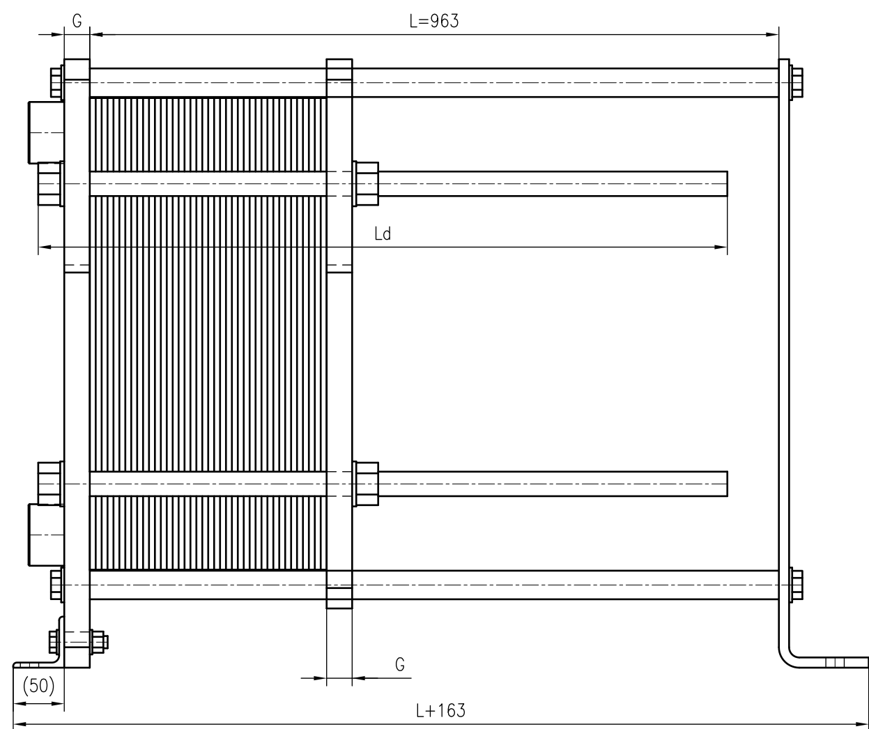
Side view
