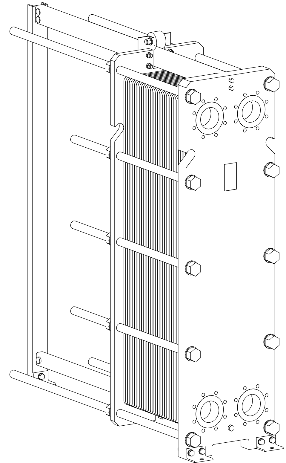
Isometric view
