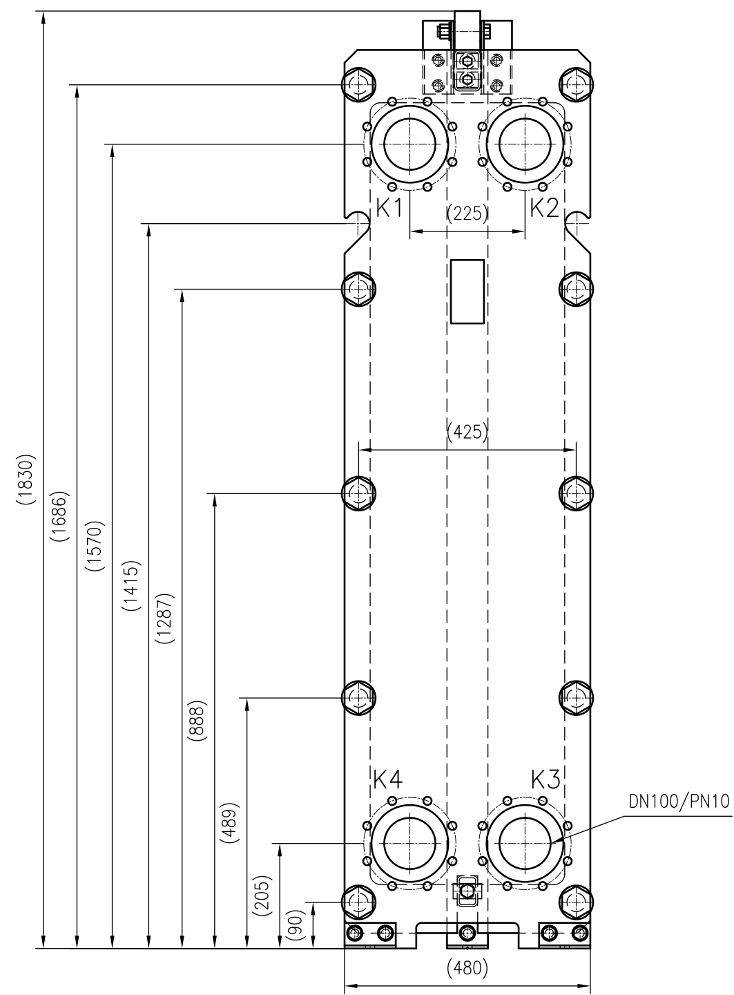
Front view
