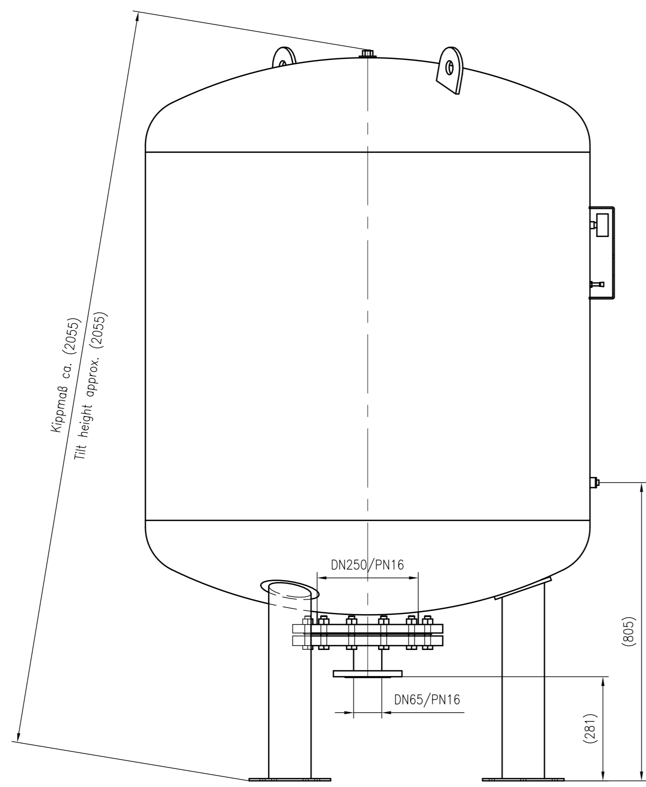
Side view
