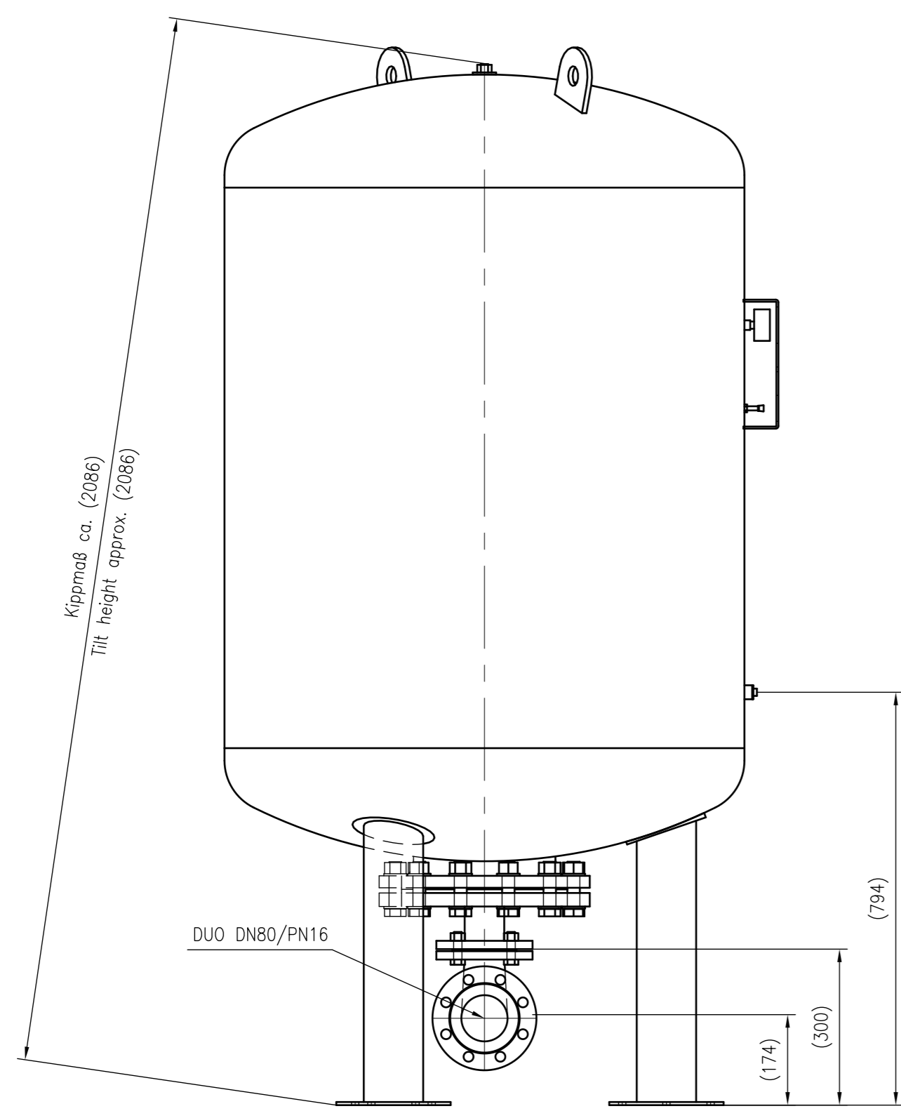
Side view
