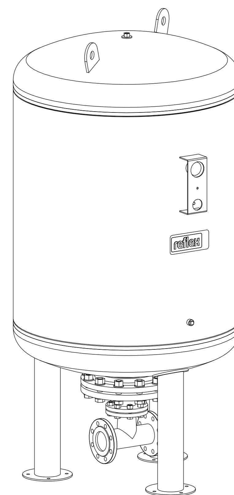
Isometric view
