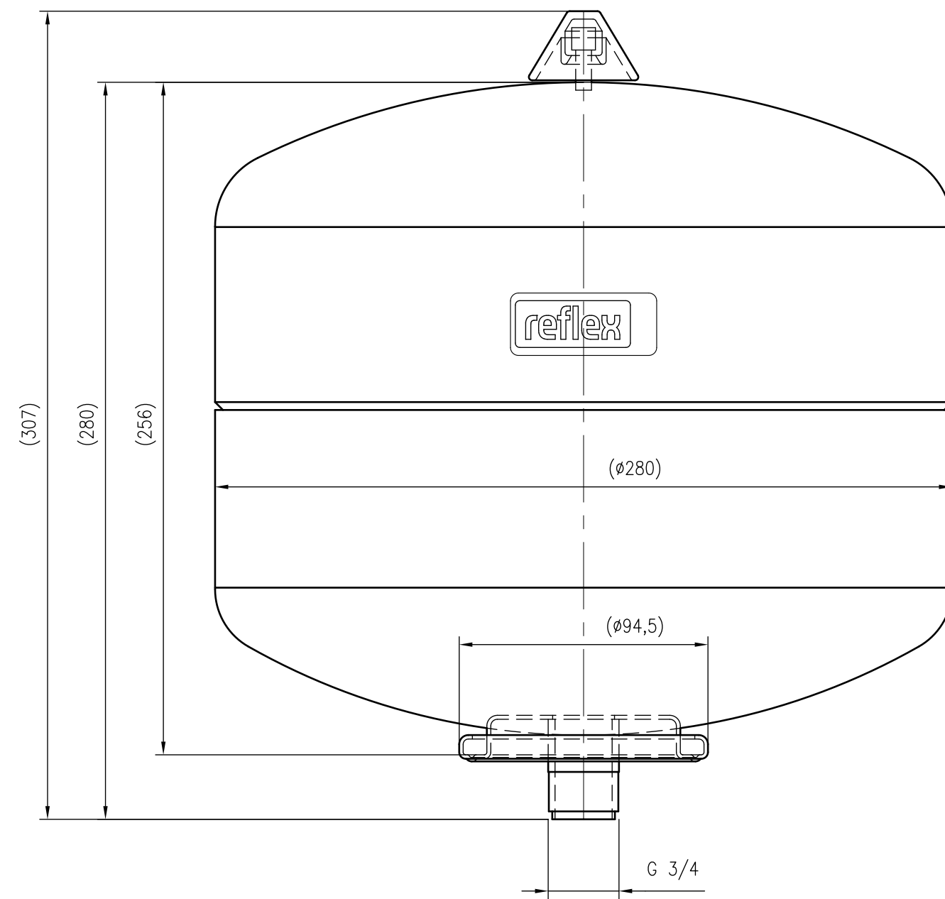
Front view
