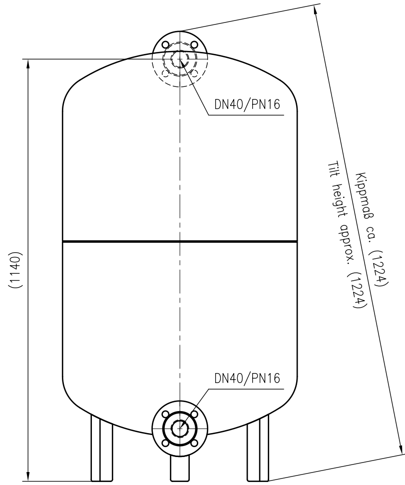
Side view
