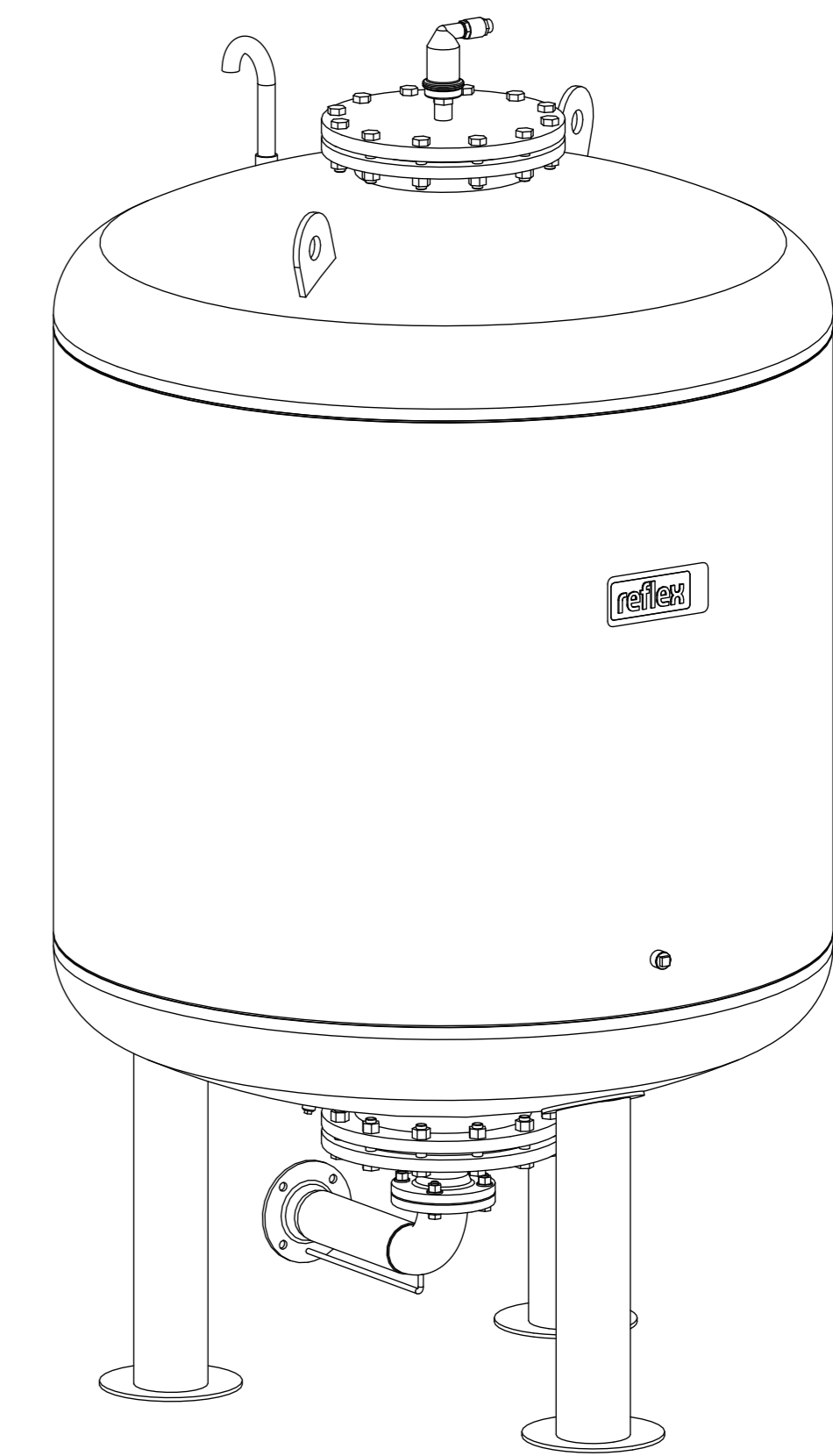
Isometric view
