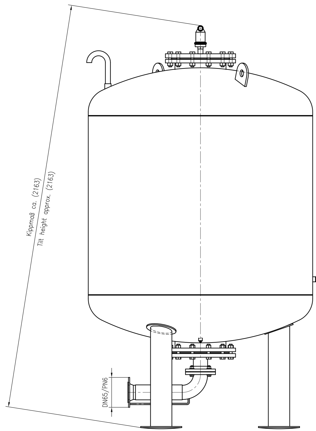
Side view
