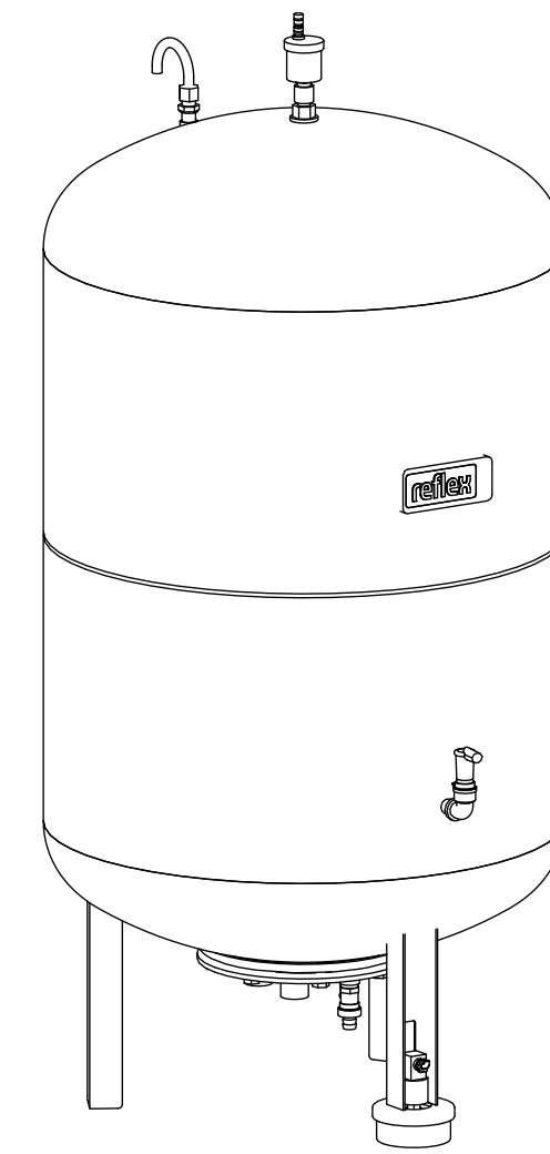
Isometric view
