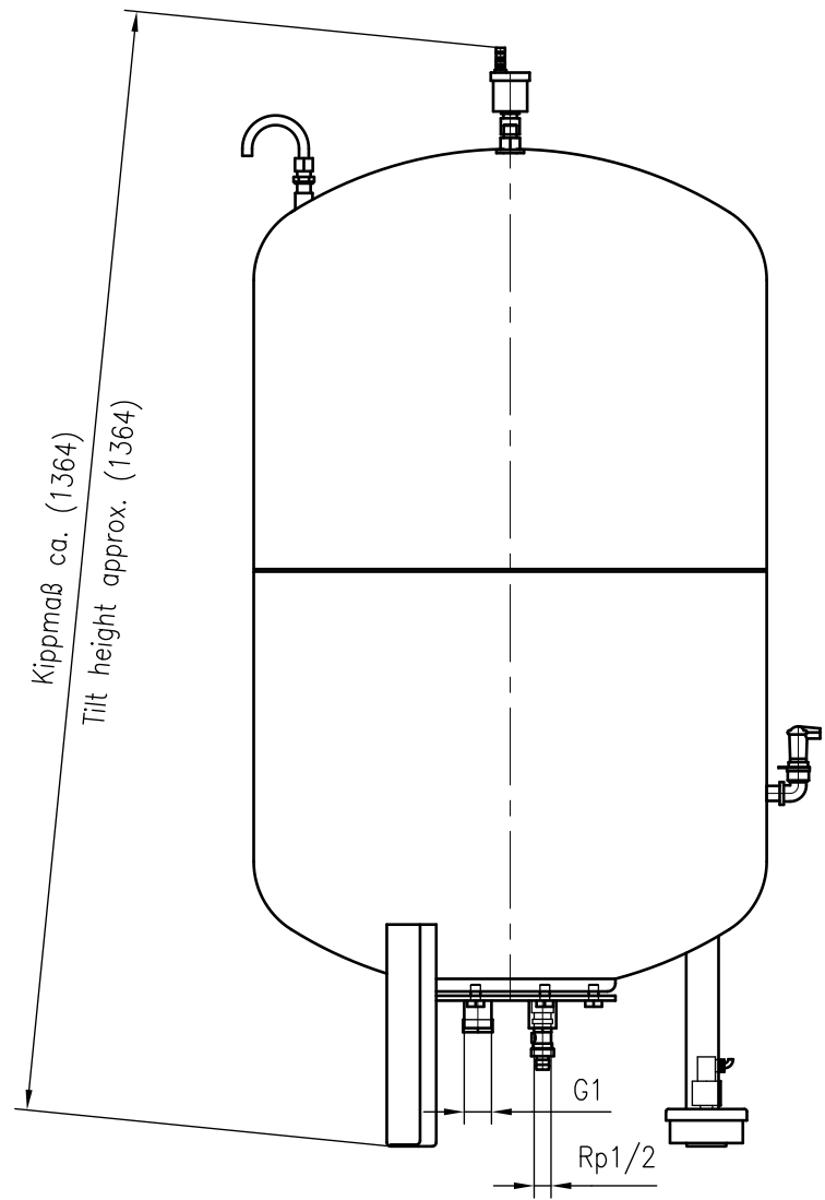
Side view
