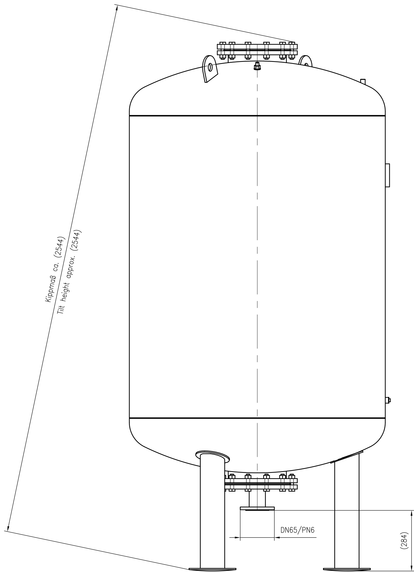
Side view
