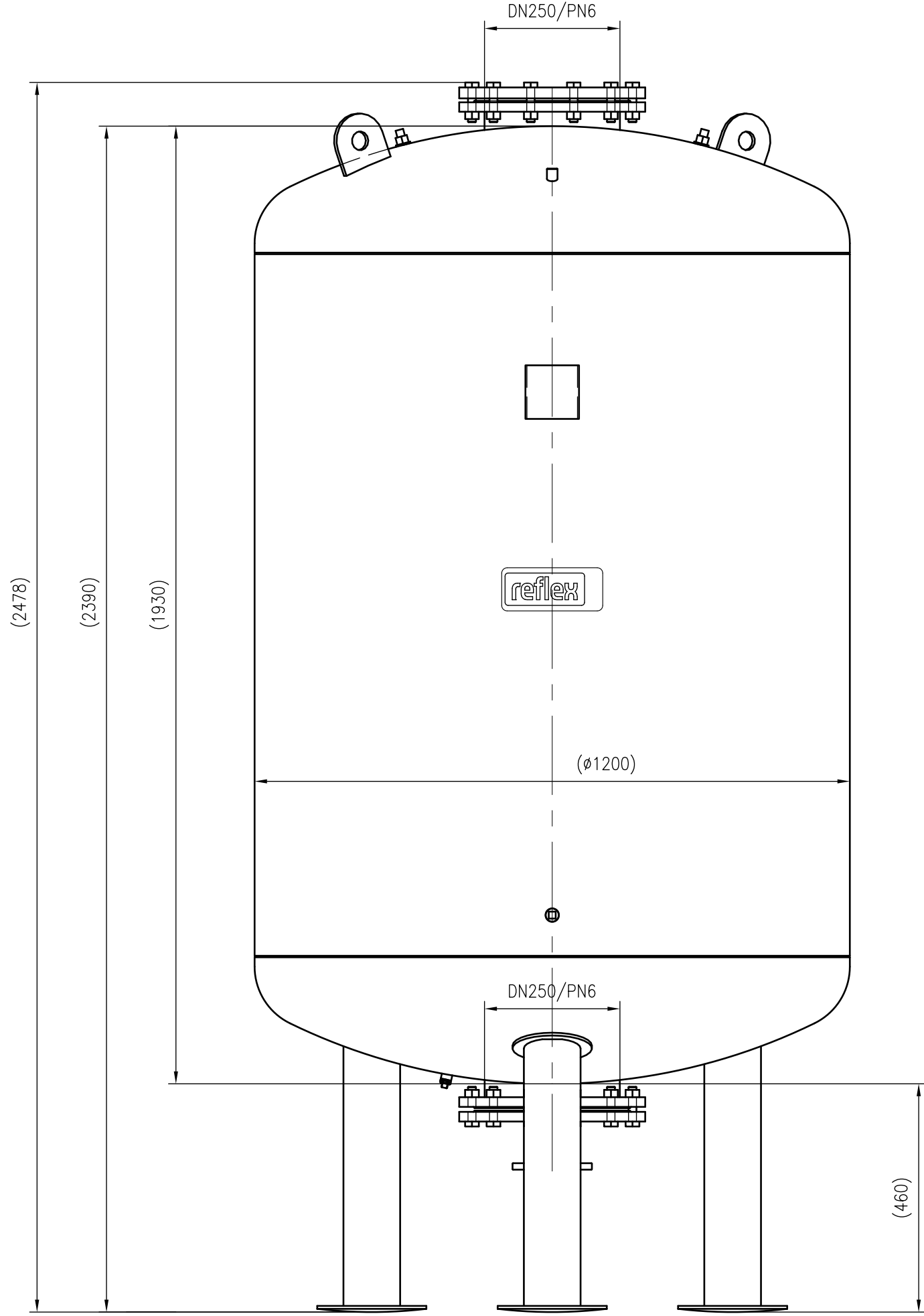
Front view
