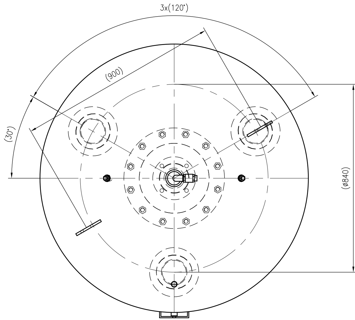
Top view
