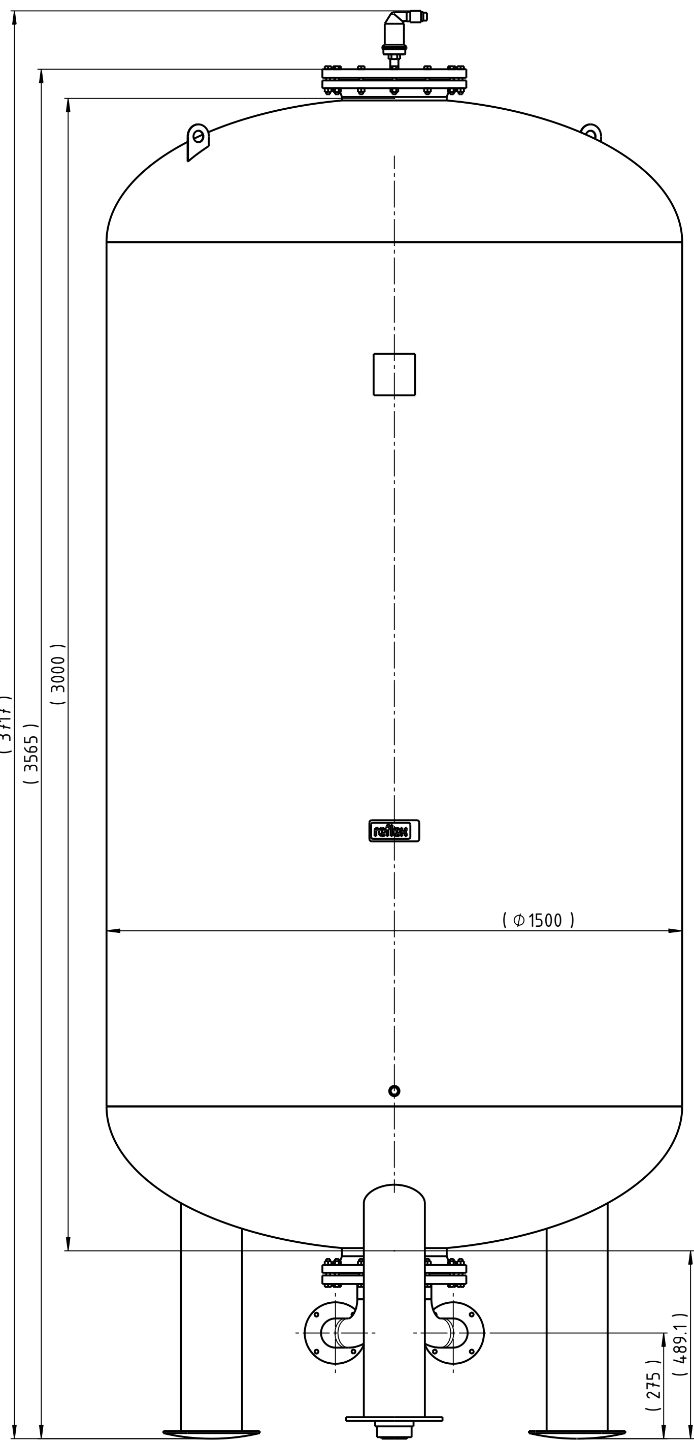
Front view
