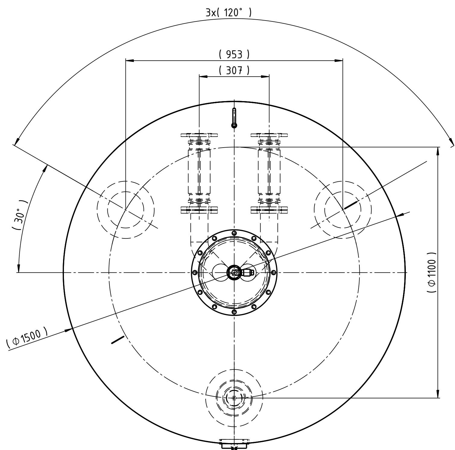
Top view
