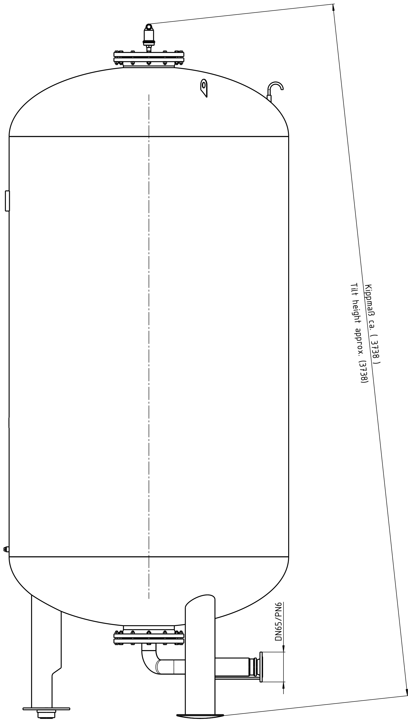
Right view
