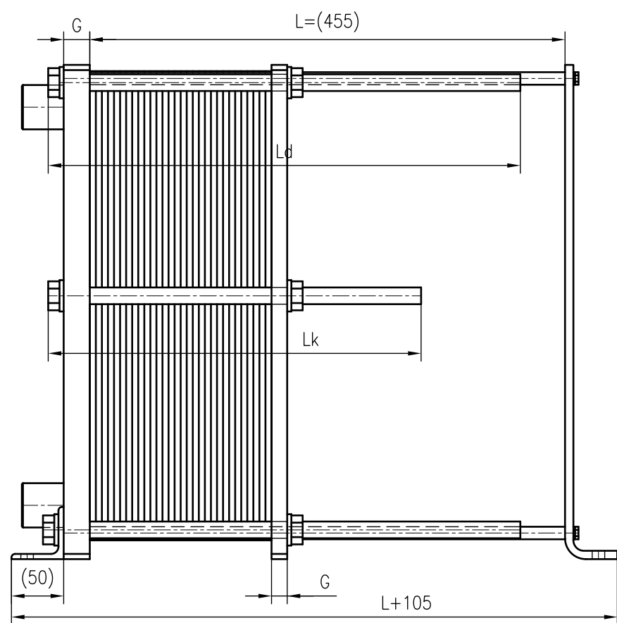
Side view
