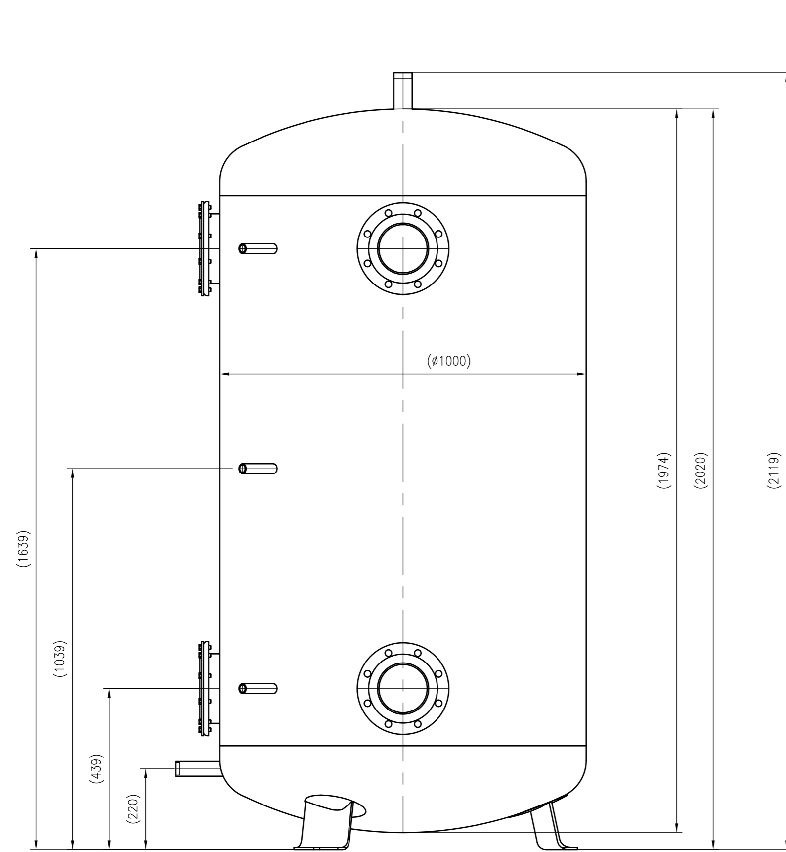
Side view
