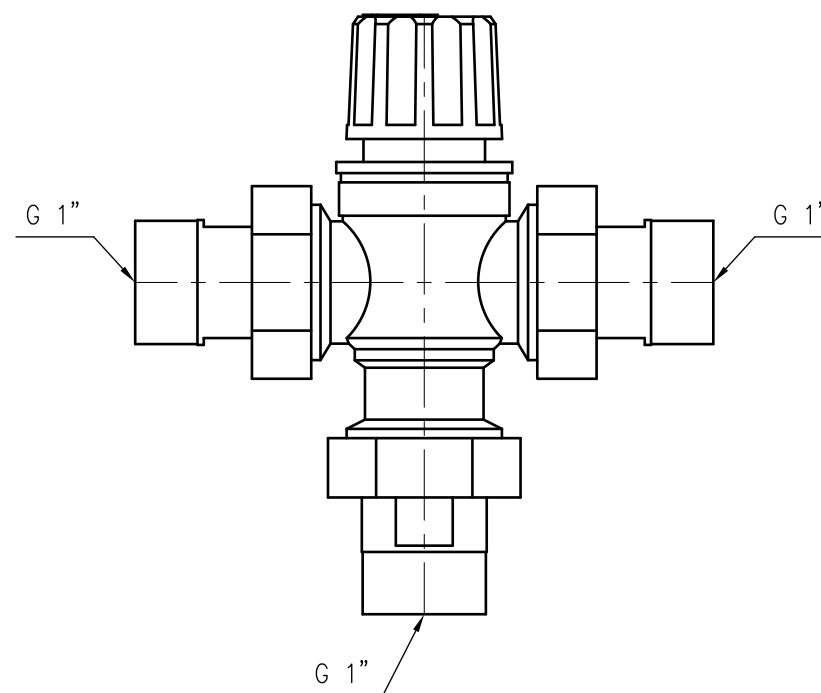
Front view
