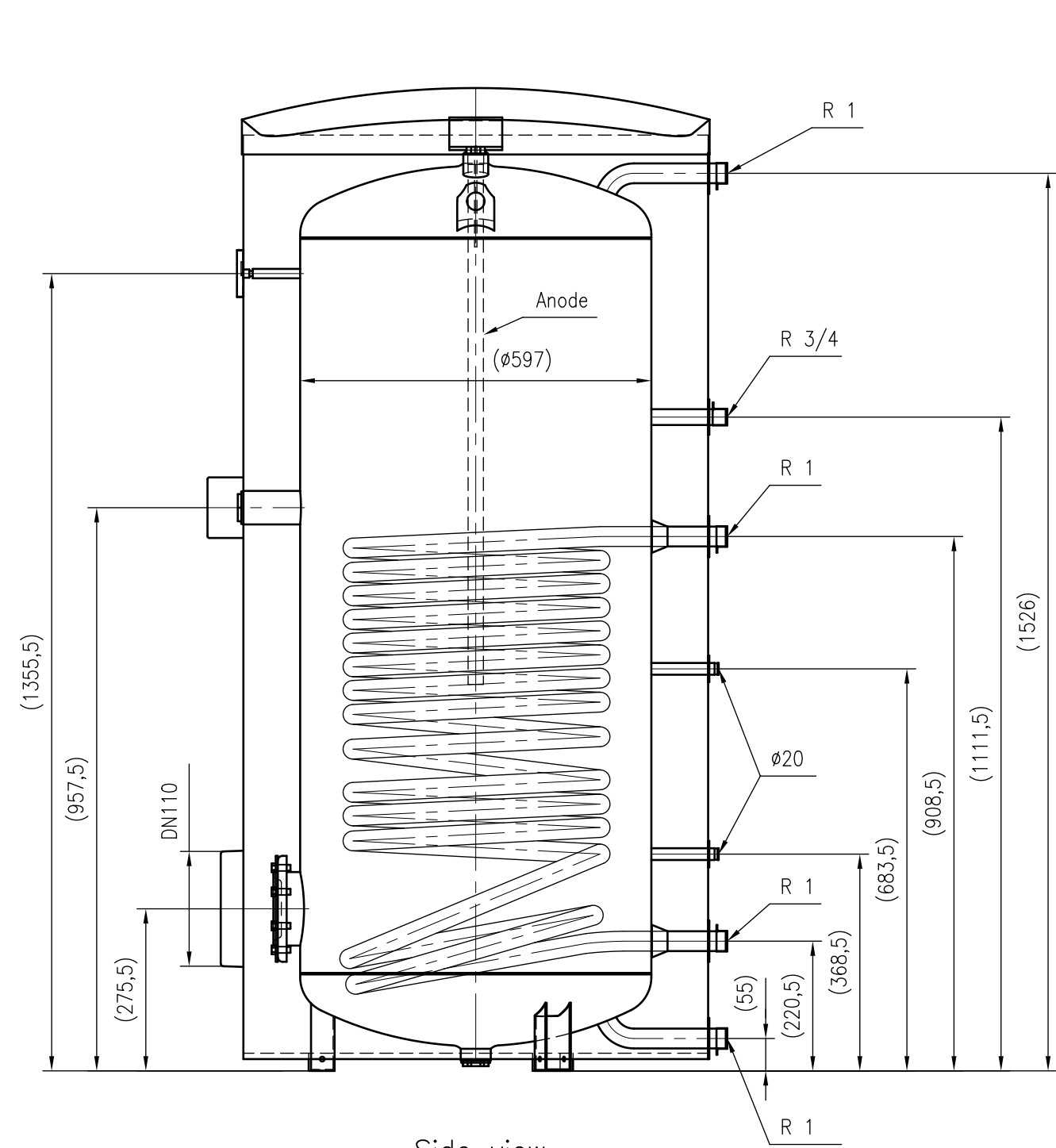
Side view
