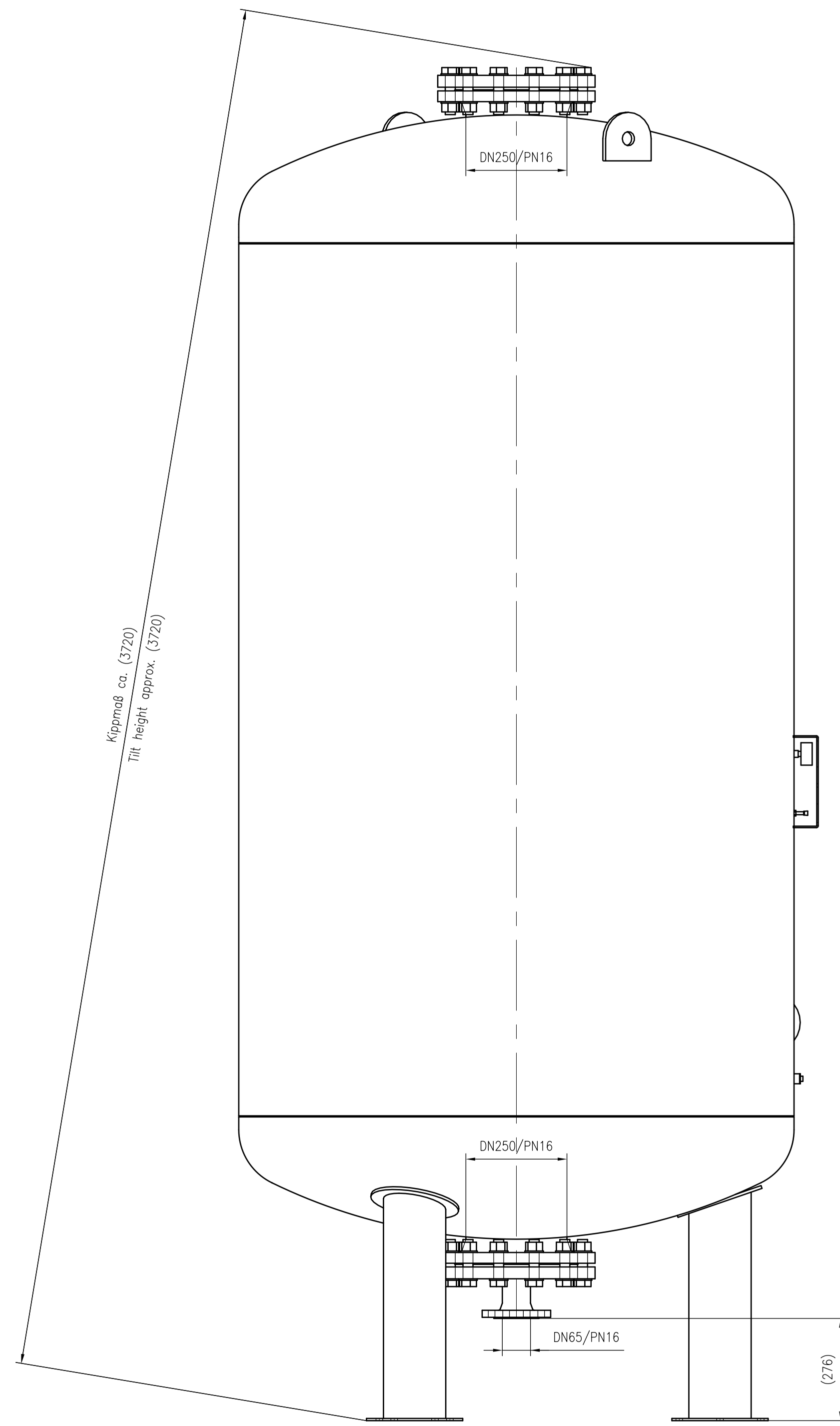
Side view
