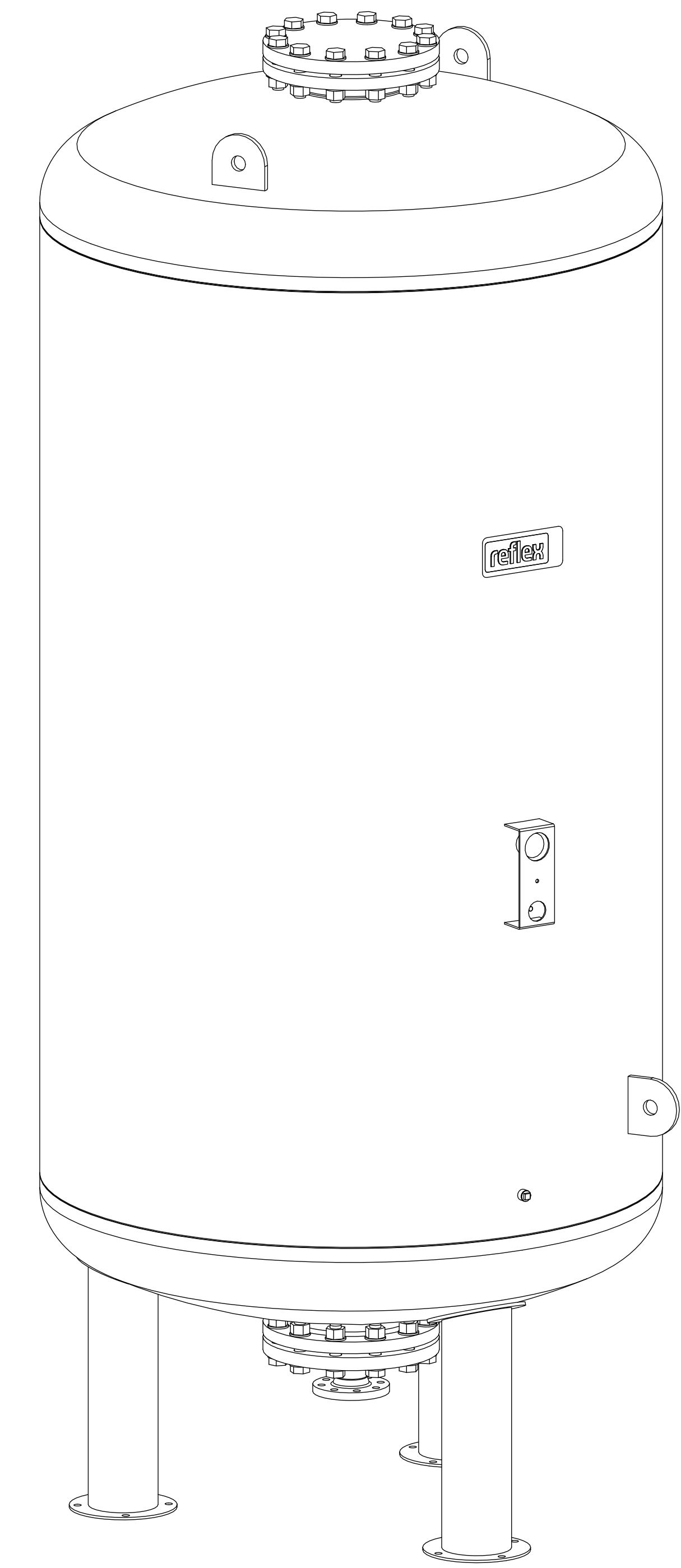
Isometric view
