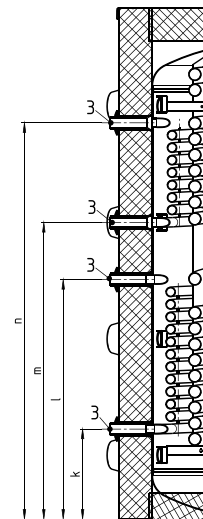
Section view C-C
