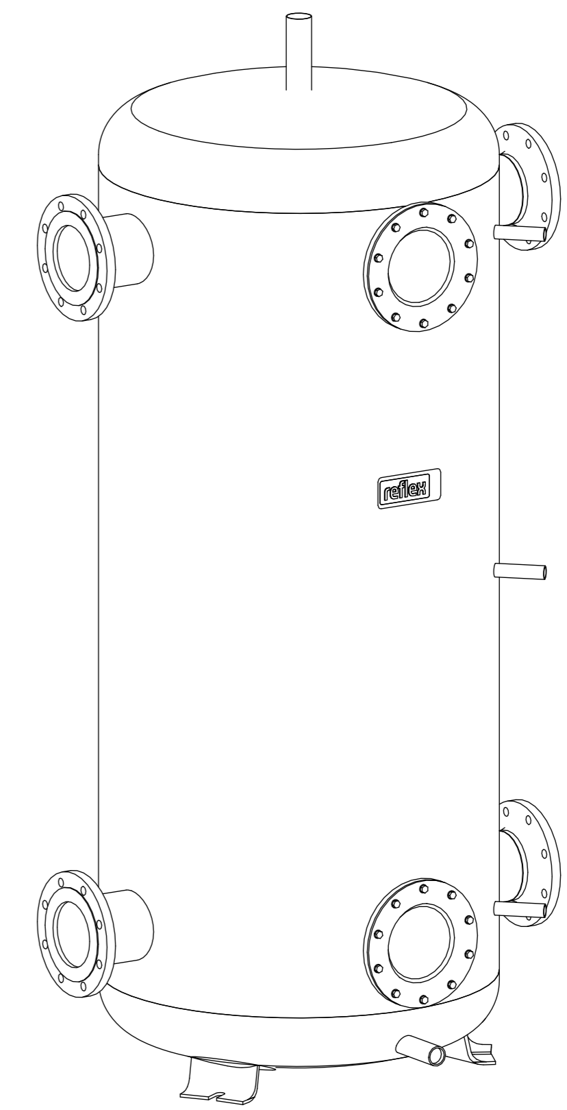
Isometric view
