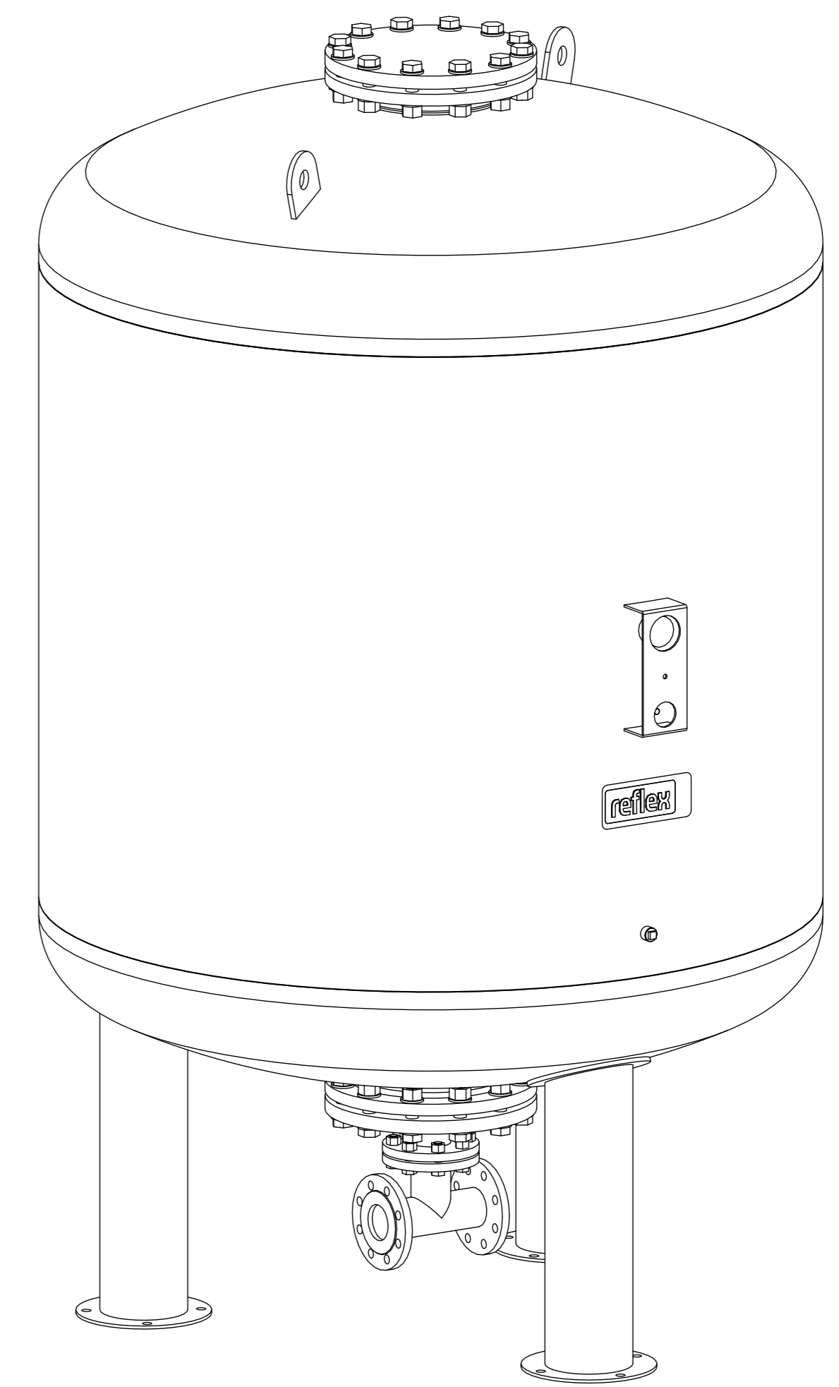
Isometric view
