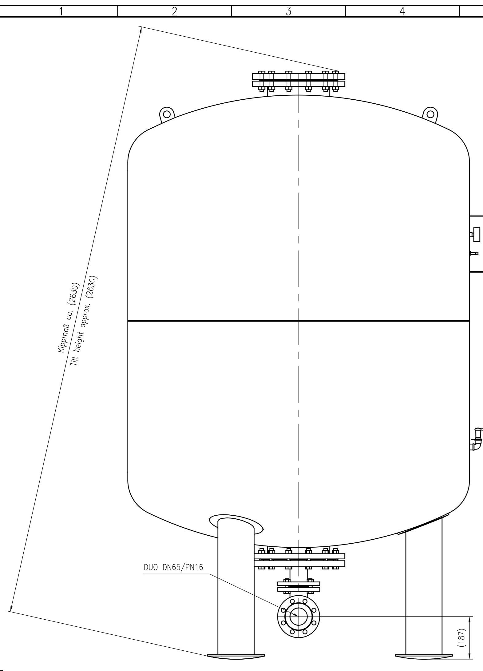
Side view
