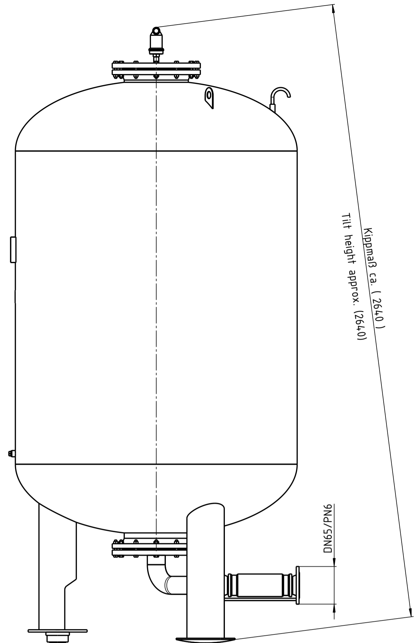
Right view
